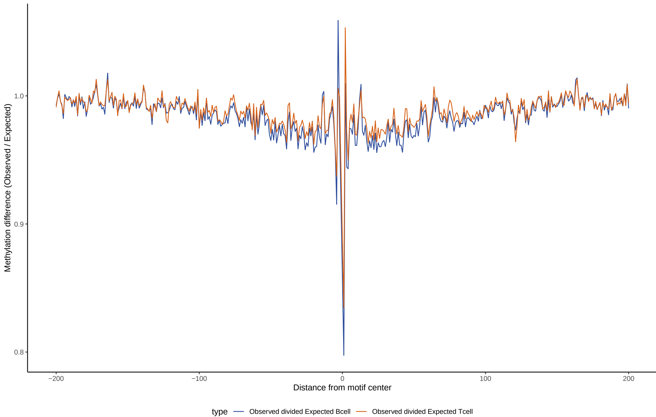
TF footprint difference for TAL1::TCF3
