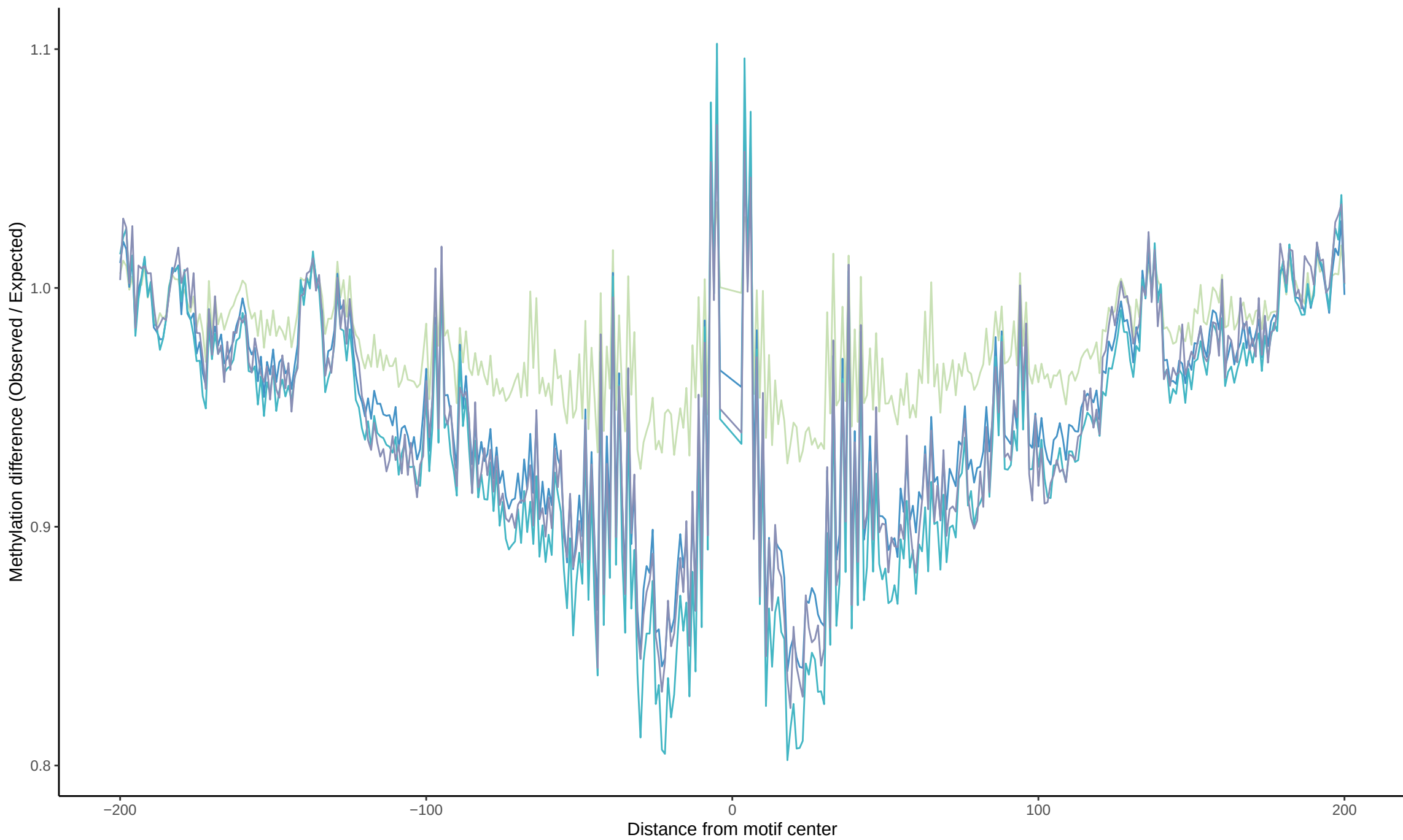
TF footprint difference for FOSL2
