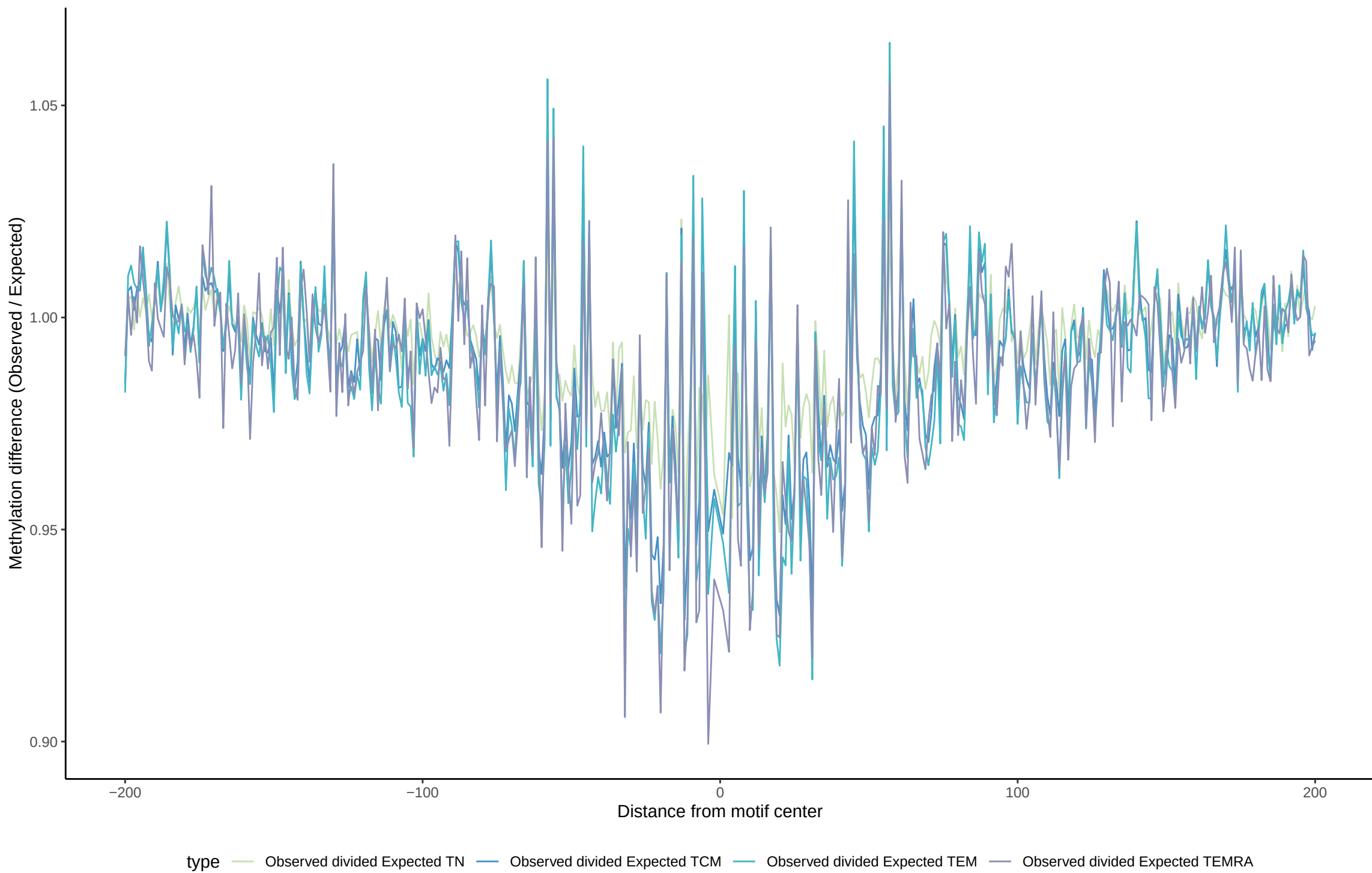
TF footprint difference for JUN
