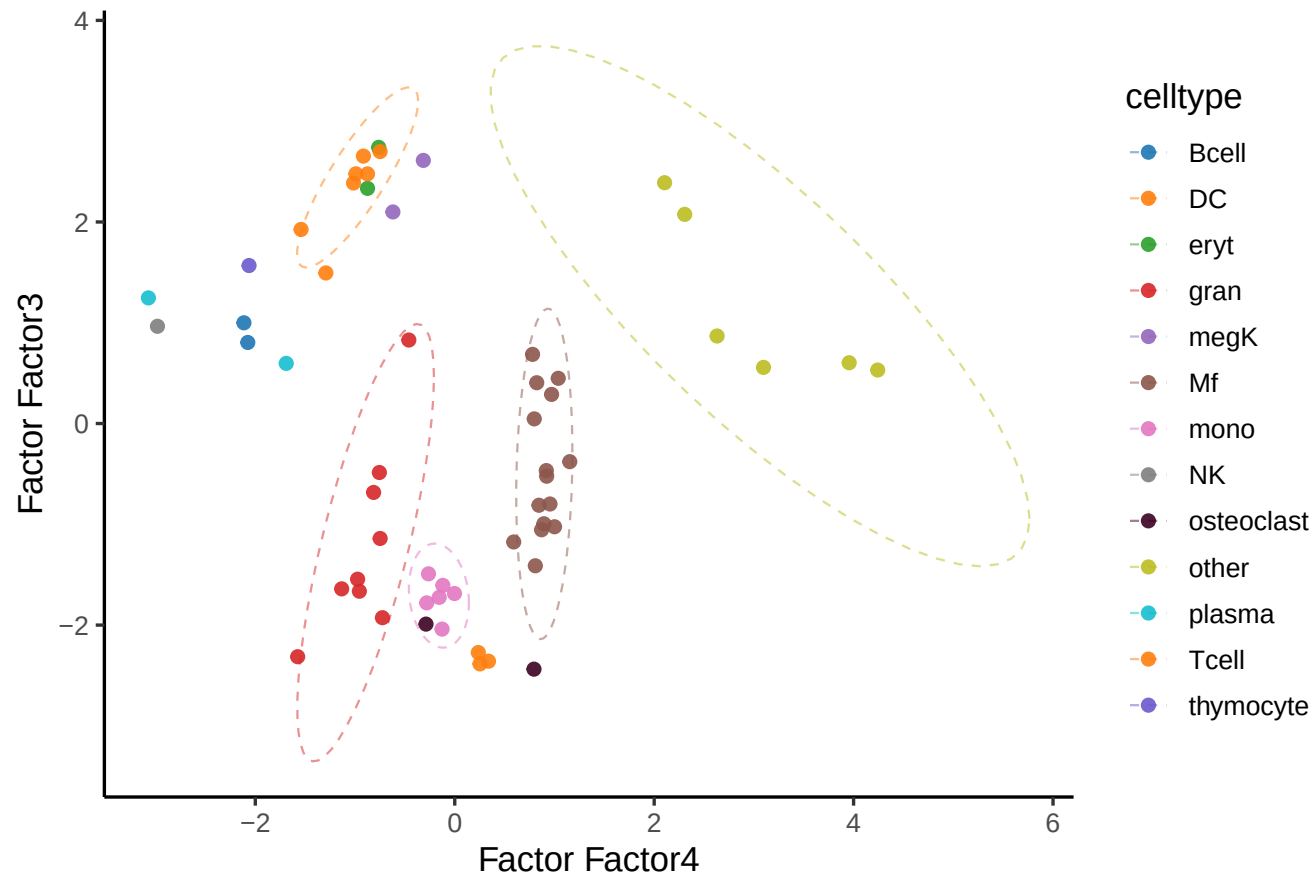
MOFA: Factor Factor4 vs Factor3 (colored by celltype)
