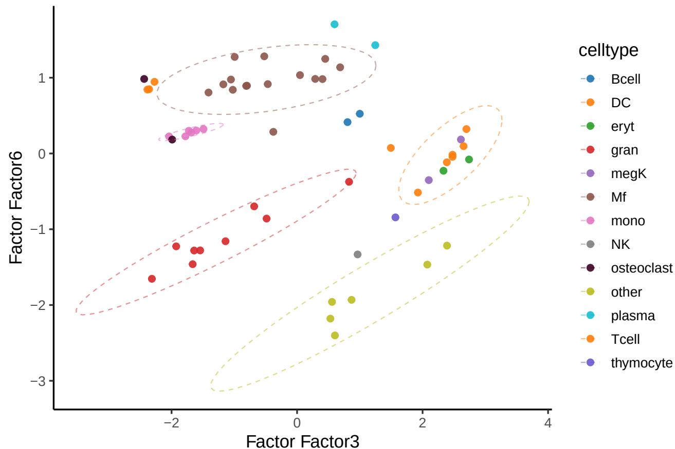
MOFA: Factor Factor3 vs Factor6 (colored by celltype)
