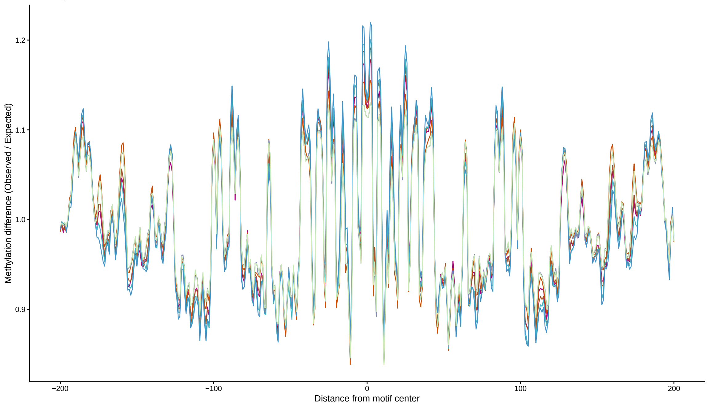
TF footprint difference for E2F2
