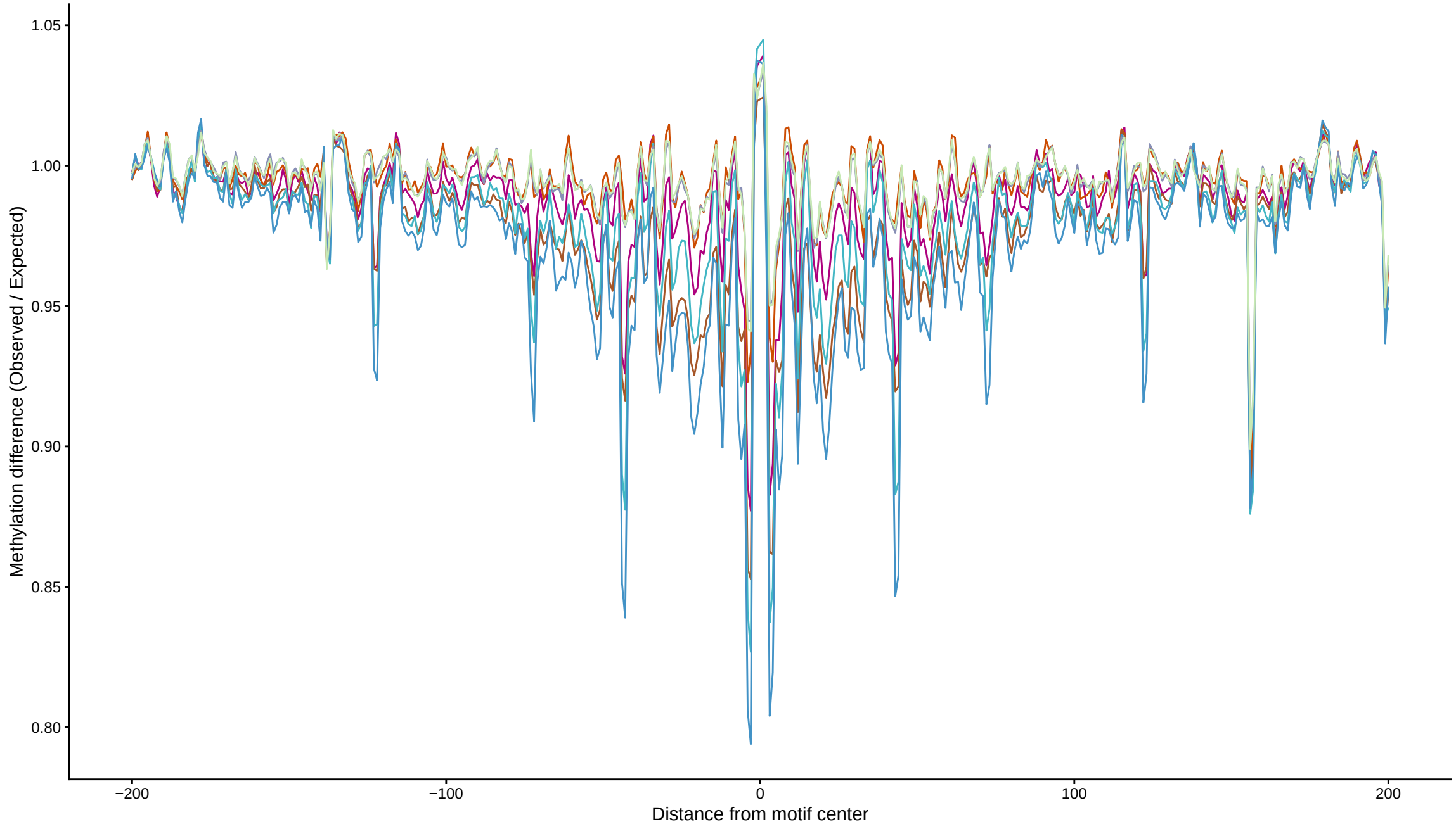
TF footprint difference for EOMES
