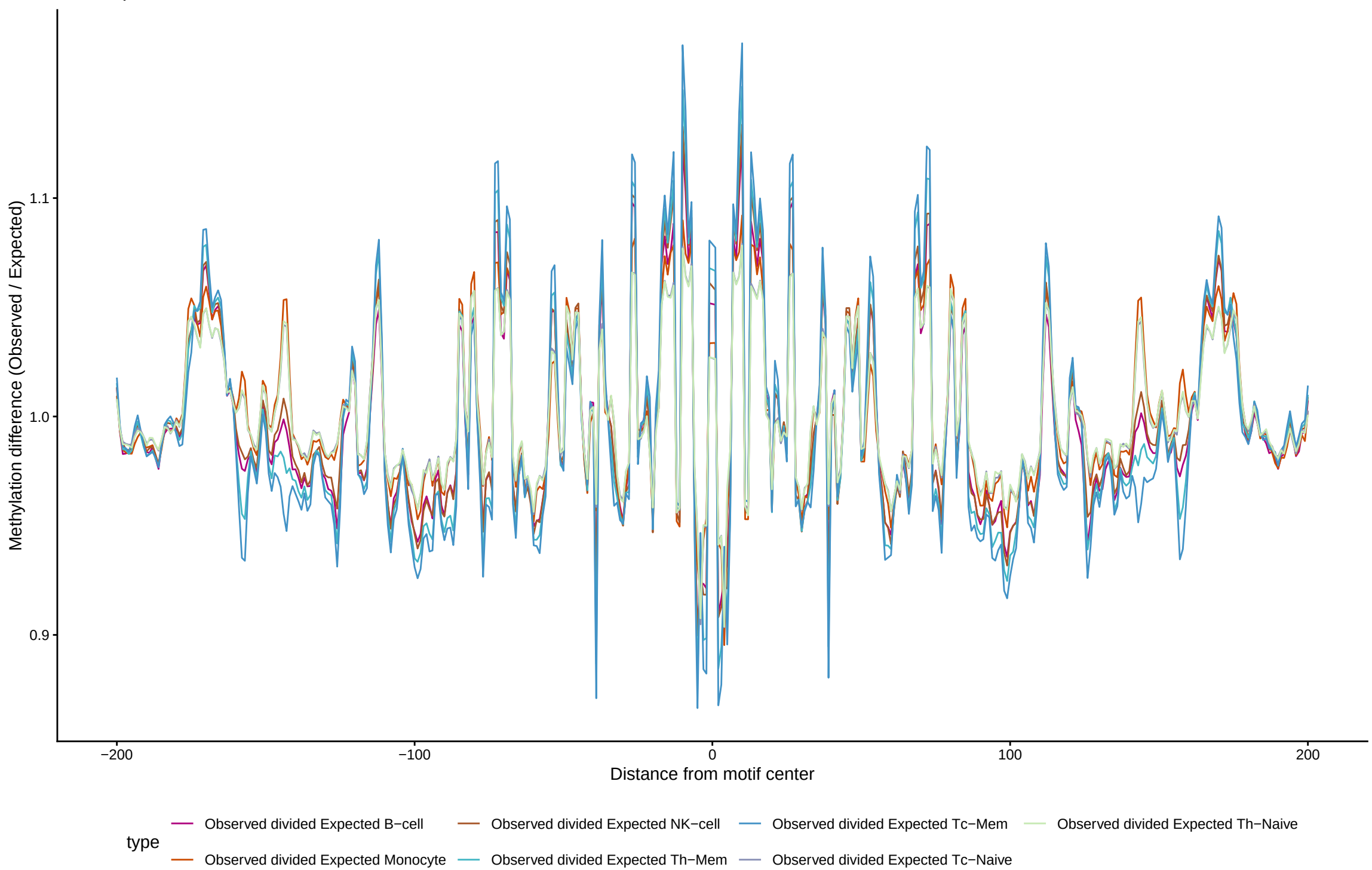
TF footprint difference for ESR1
