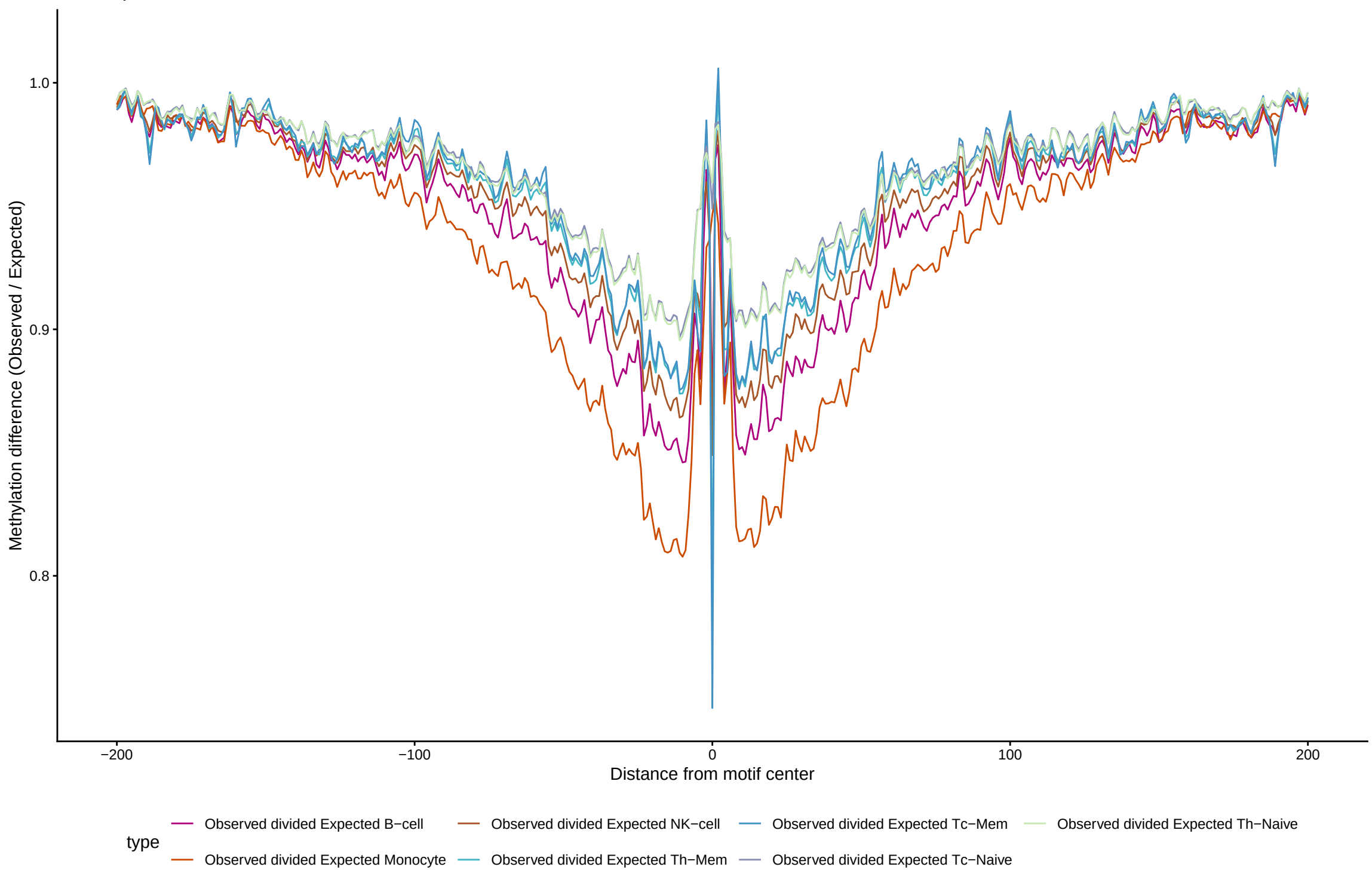
TF footprint difference for SPIB
