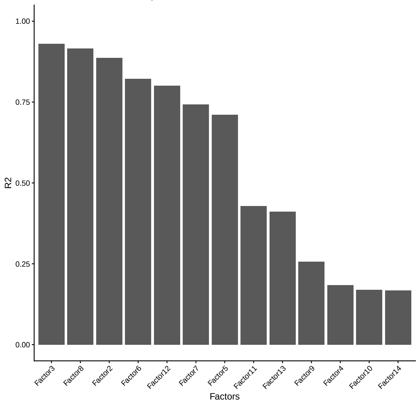
R2 values of MOFA analysis
