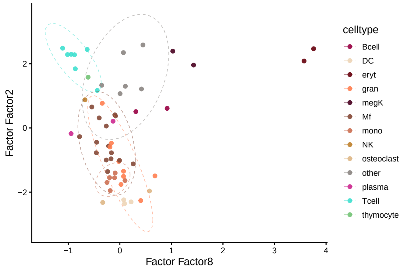
MOFA: Factor Factor8 vs Factor2 (colored by celltype)
