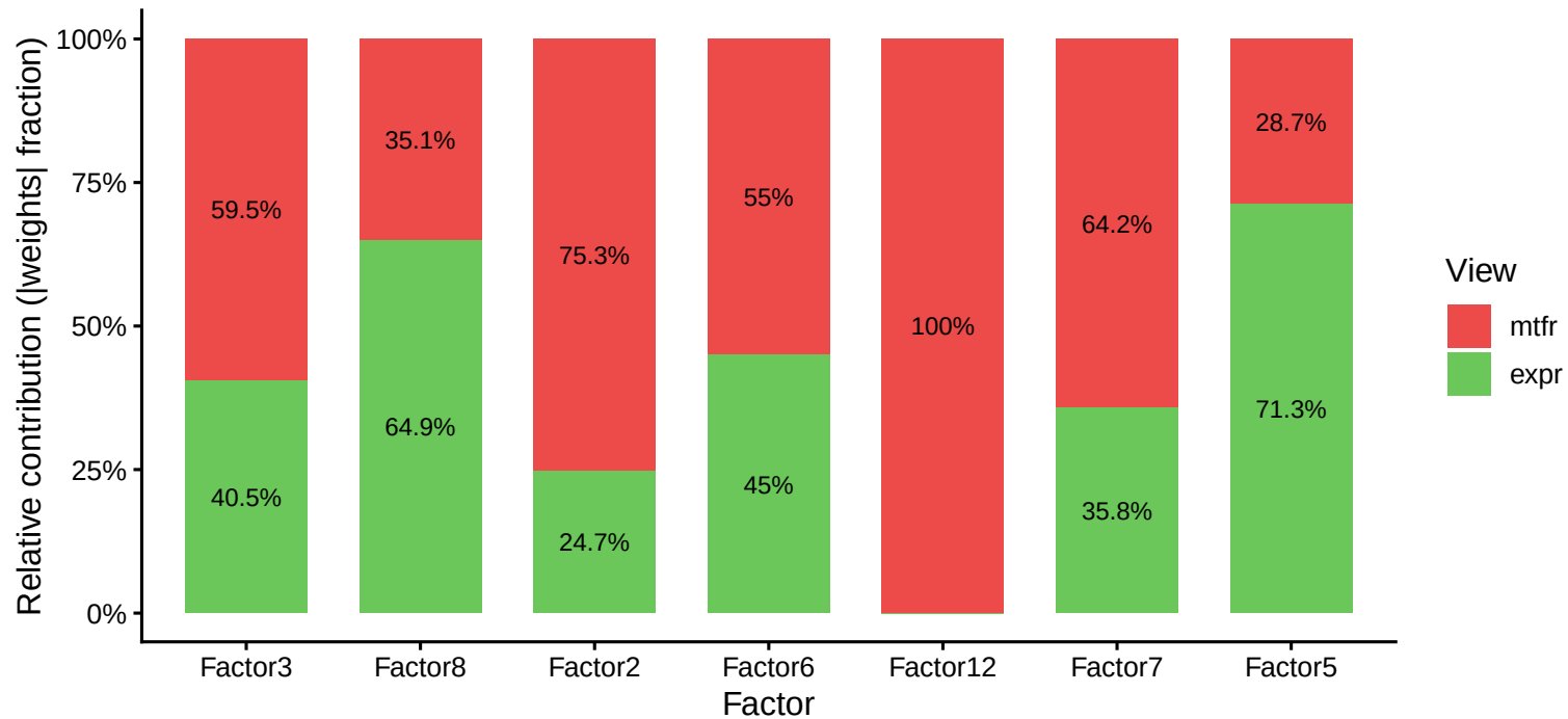
Modality contribution per factor (weights-based)
