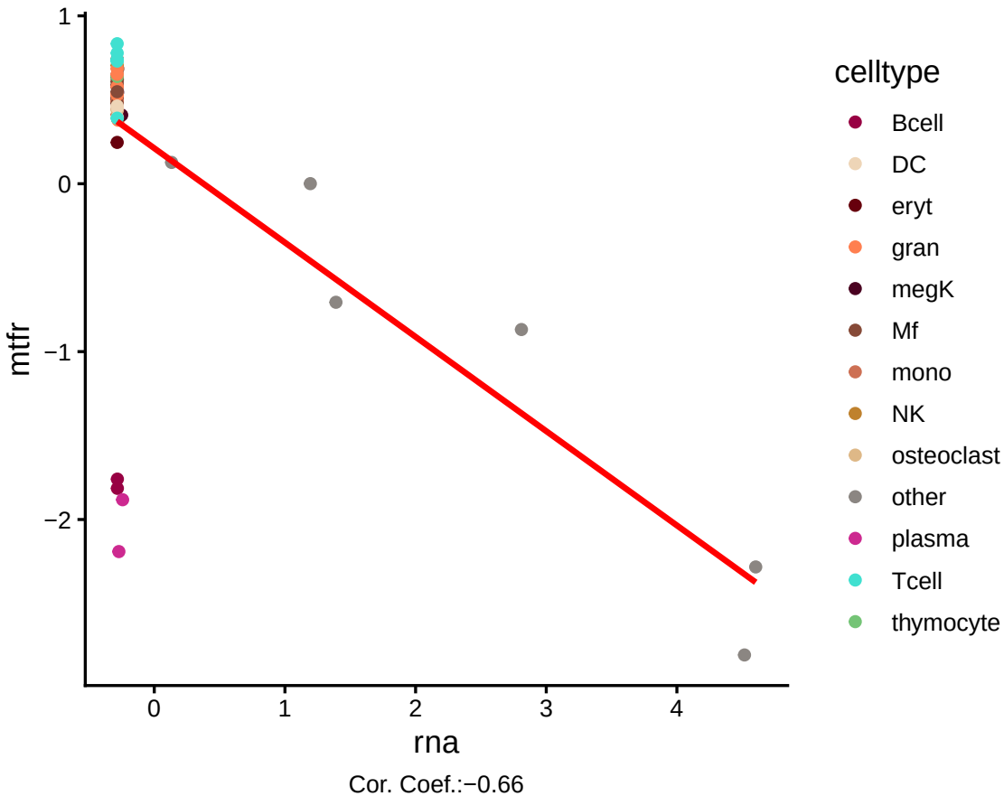
TF Activity Correlation (rna vs mtfr) for EBF3
