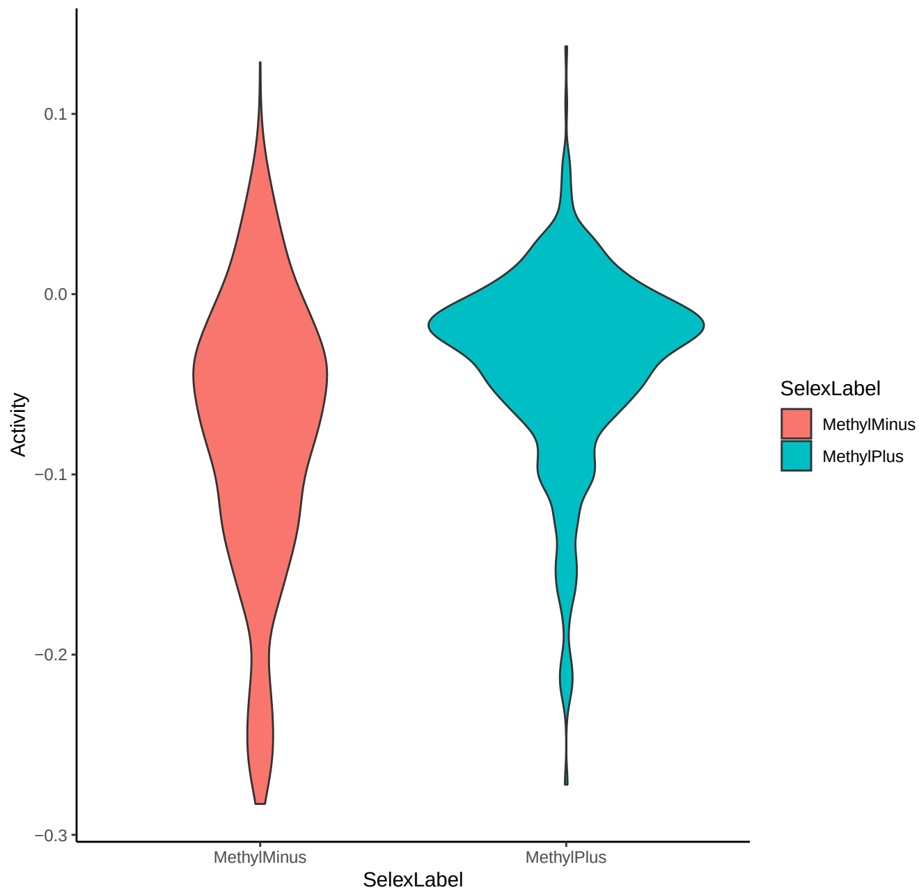
TF activity by SELEX label across plasma
