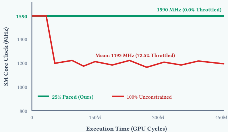
Panel A: SM Core Clock Stability (MHz)
