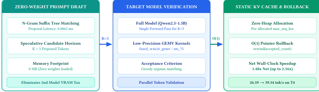
Figure 5: Unified Speculative Serving Engine Architecture. Pre-allocated StaticKVCache with O(1) rollback and zero-weight n -gram PromptLookupDraftEngine eliminate secondary model VRAM overhead, delivering a 1.48x net wall-clock speedup on Tesla T4.
