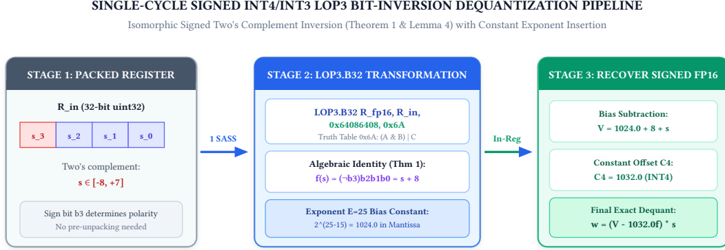
Figure 1: Single-Cycle Signed Sub-Byte LOP3 Dequantization Pipeline. The LOP3.B32 instruction applies LUT 0x6A and magic constant 0x64086408, mapping two's complement signed nibbles directly into biased FP16 mantissas in 1 SASS cycle.
