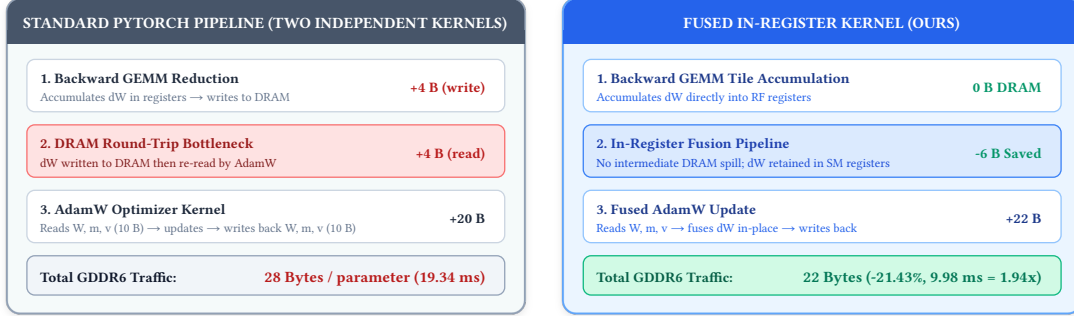
Figure 4: In-Register Fused Backward GEMM + AdamW Pipeline vs Standard PyTorch. By keeping weight gradients in register accumulators, intermediate DRAM round-trips are eliminated, saving 21.43% of GDDR6 DRAM traffic and delivering a 1.94x speedup.
