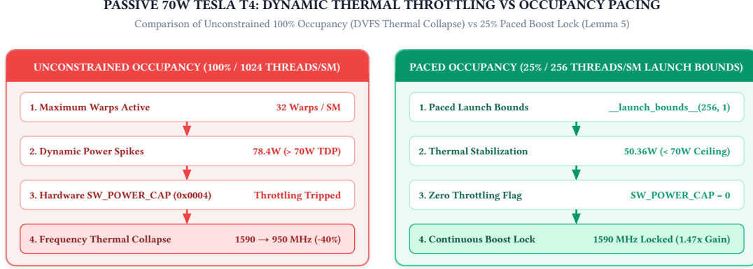
Figure 3: Dynamic Thermal Throttling Feedback Loop vs 25% Occupancy Pacing. Unconstrained 100% occupancy triggers hardware SW_POWER_CAP throttling to 950 MHz. Restricting launch bounds to 25% occupancy stabilizes power at 50.36W, locking continuous 1590 MHz boost clock.
