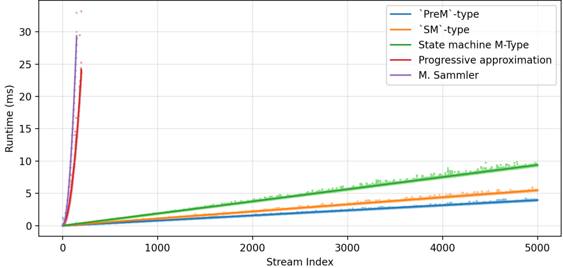
Figure 29: Cumulative performance for stream destructuring
