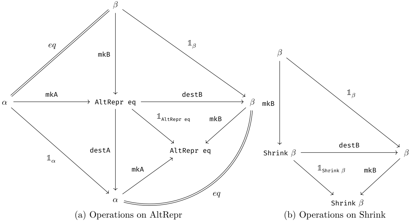
Figure 24: Universe transforming types.
