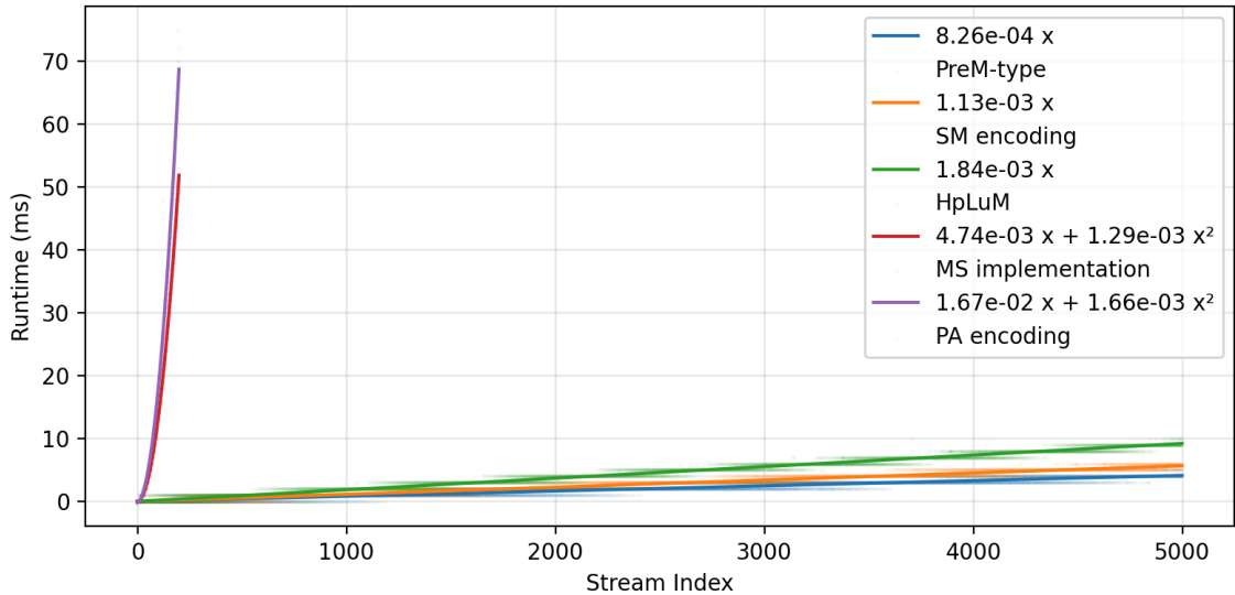
Figure 21: Performance of PA, HpLuM , and SM & PreM representation
