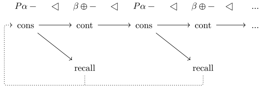
Figure 20: Choice points for a producing a stream
