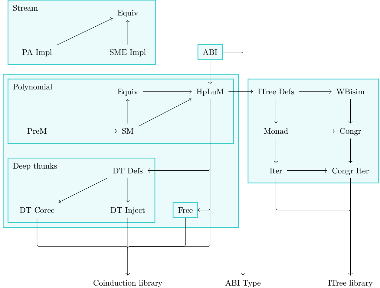
Figure 12: Birds-eye view of components of the project
