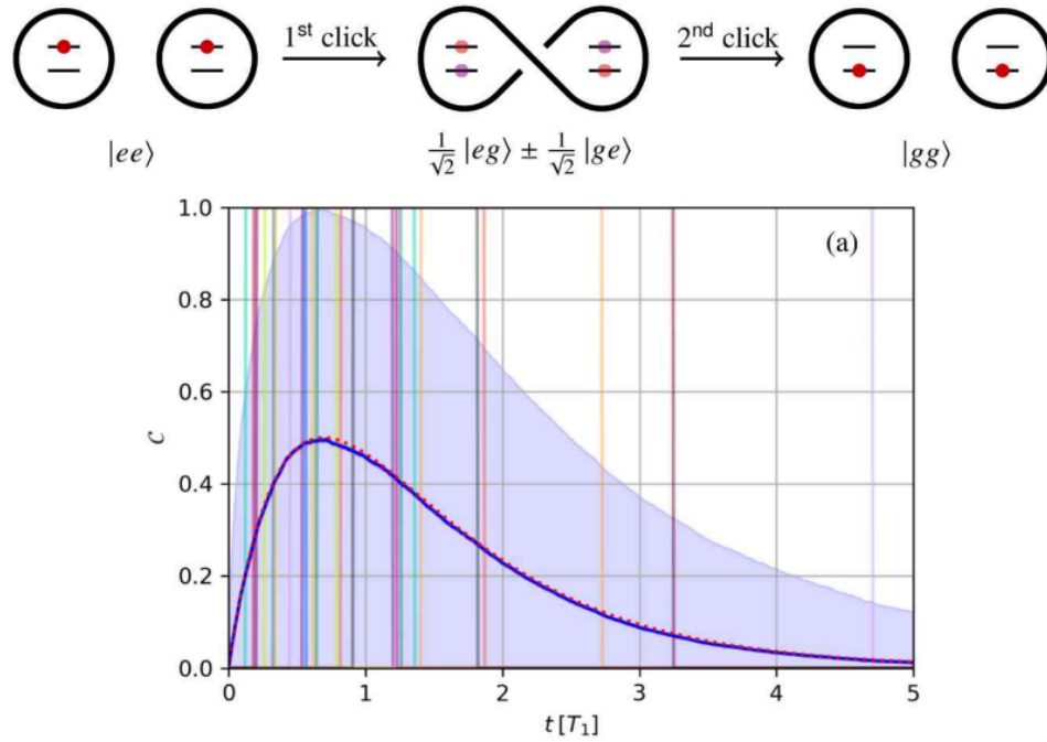
Figure 3.2: Ideal photodetection dynamics for two emitters initially prepared in |ee\rangle . In the lower panel, the horizontal axis reports the rescaled time t/T_1 , while the vertical axis shows the concurrence C . The solid curve represents the trajectory-averaged concurrence, as given by Eq. (3.6), whereas the vertical colored lines denote the click times for different individual trajectories. The upper panel illustrates the corresponding jump mechanism.
