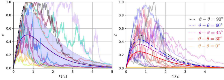
Figure 3.3: Homodyne entanglement generation starting from |ee\rangle . In both panels, the horizontal axis reports the rescaled time t/T_1 , while the vertical axis shows the concurrence C . Left panel: individual diffusive trajectories and corresponding trajectory-averaged concurrence for the optimal homodyne phases. Right panel: average concurrence for different relative phase differences \vartheta - \theta . The maximal entanglement yield is obtained for |\vartheta - \theta| = \pi/2 , while deviations from this condition reduce the concurrence by progressively restoring which-path distinguishability.
