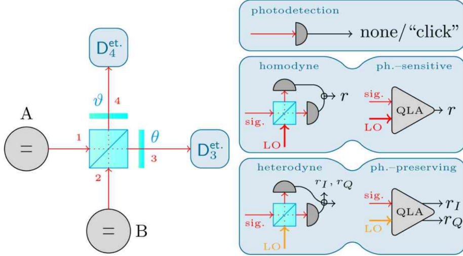
Figure 3.1: Schematic representation of the measurement setup. Two remote qubits emit into two independent output modes, which are mixed on a balanced beam splitter and then monitored at the two output ports. The relative phases in the two paths are controlled by phase shifters. Different choices of detection at the output, namely photodetection, homodyne, or heterodyne measurement, correspond to different unravellings of the same open-system dynamics. Adapted from Ref. [42].
