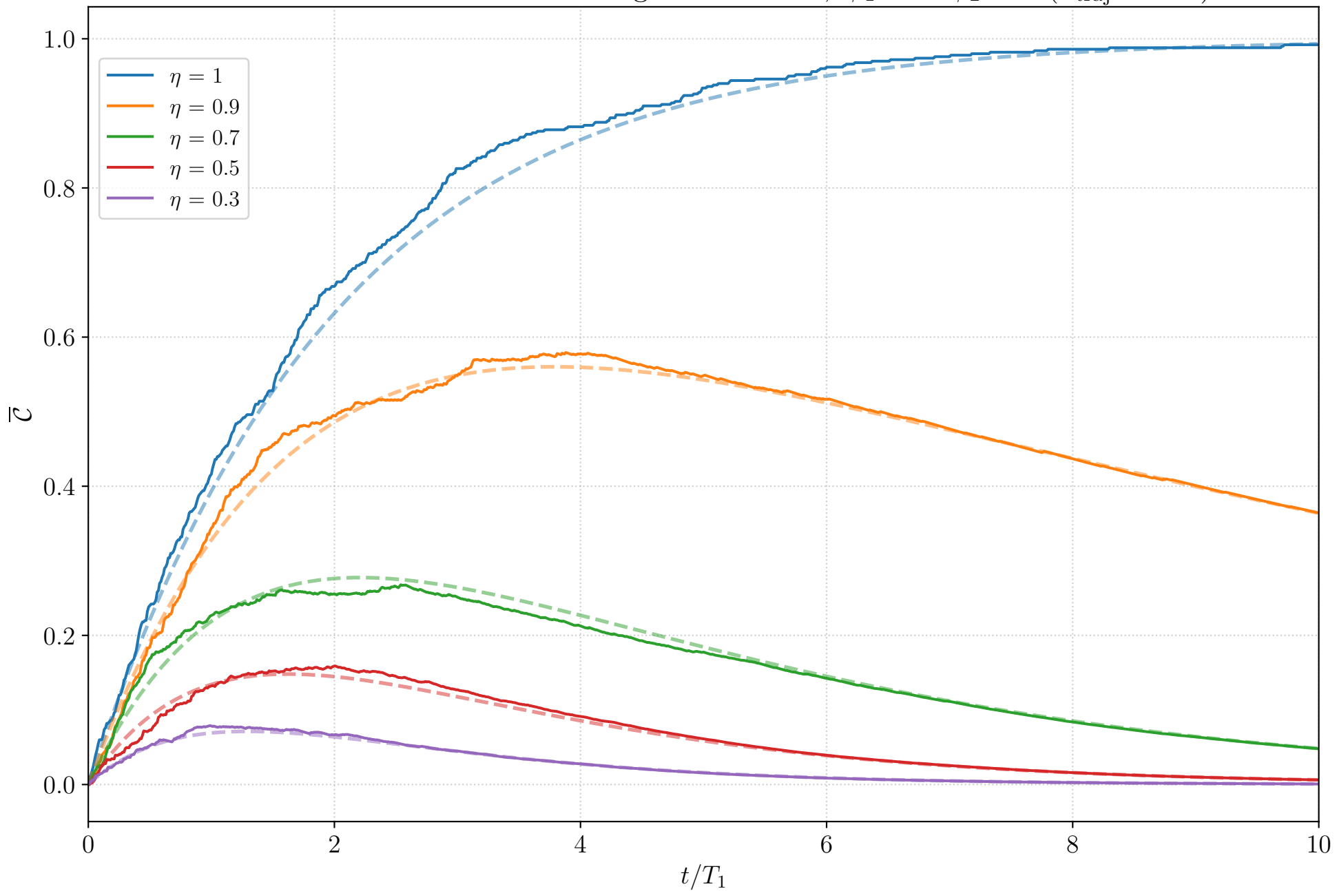
Inefficient Photodetection: Average \bar{\mathcal{C}} over time, \phi_1 = 0 \phi_2 = 0 ( n_{\text{traj}} = 500 )
