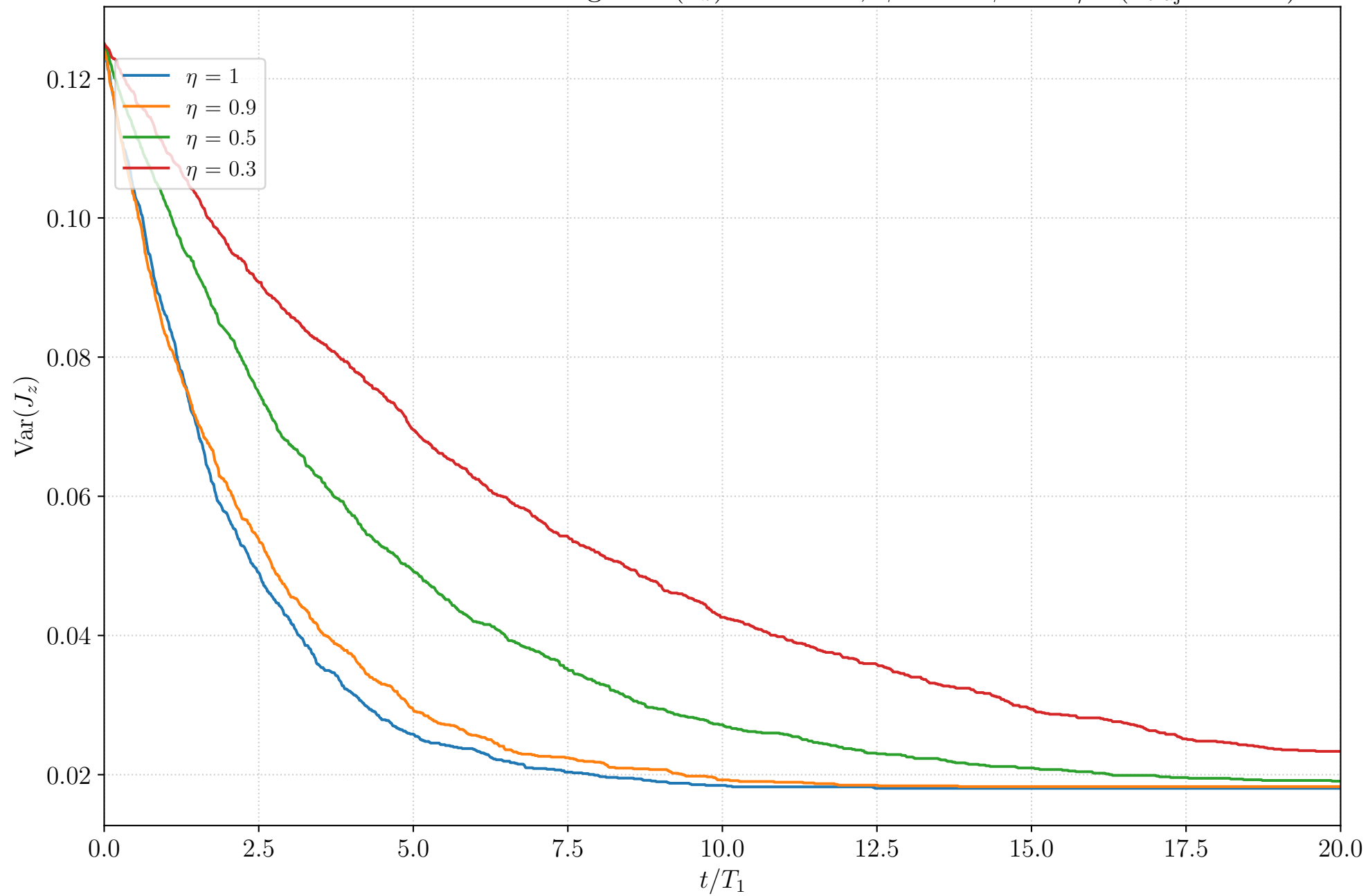
Inefficient Photodetection: Average \text{Var}(J_z) over time, \phi_1 = 0 \phi_2 = \pi/2 ( n_{\text{traj}} = 1000 )
