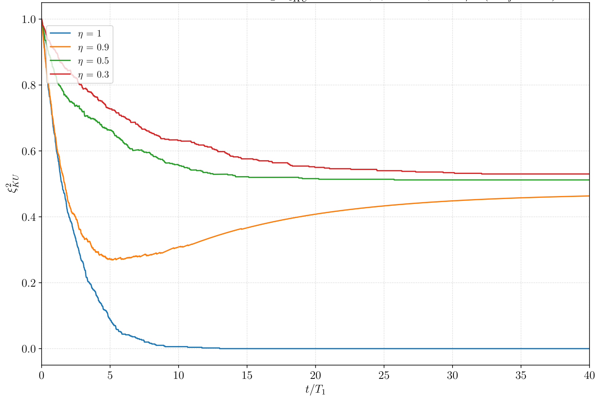
Inefficient Photodetection: Average \xi_{KU}^2 over time, \phi_1 = 0 \phi_2 = \pi/2 ( n_{\text{traj}} = 500 )
