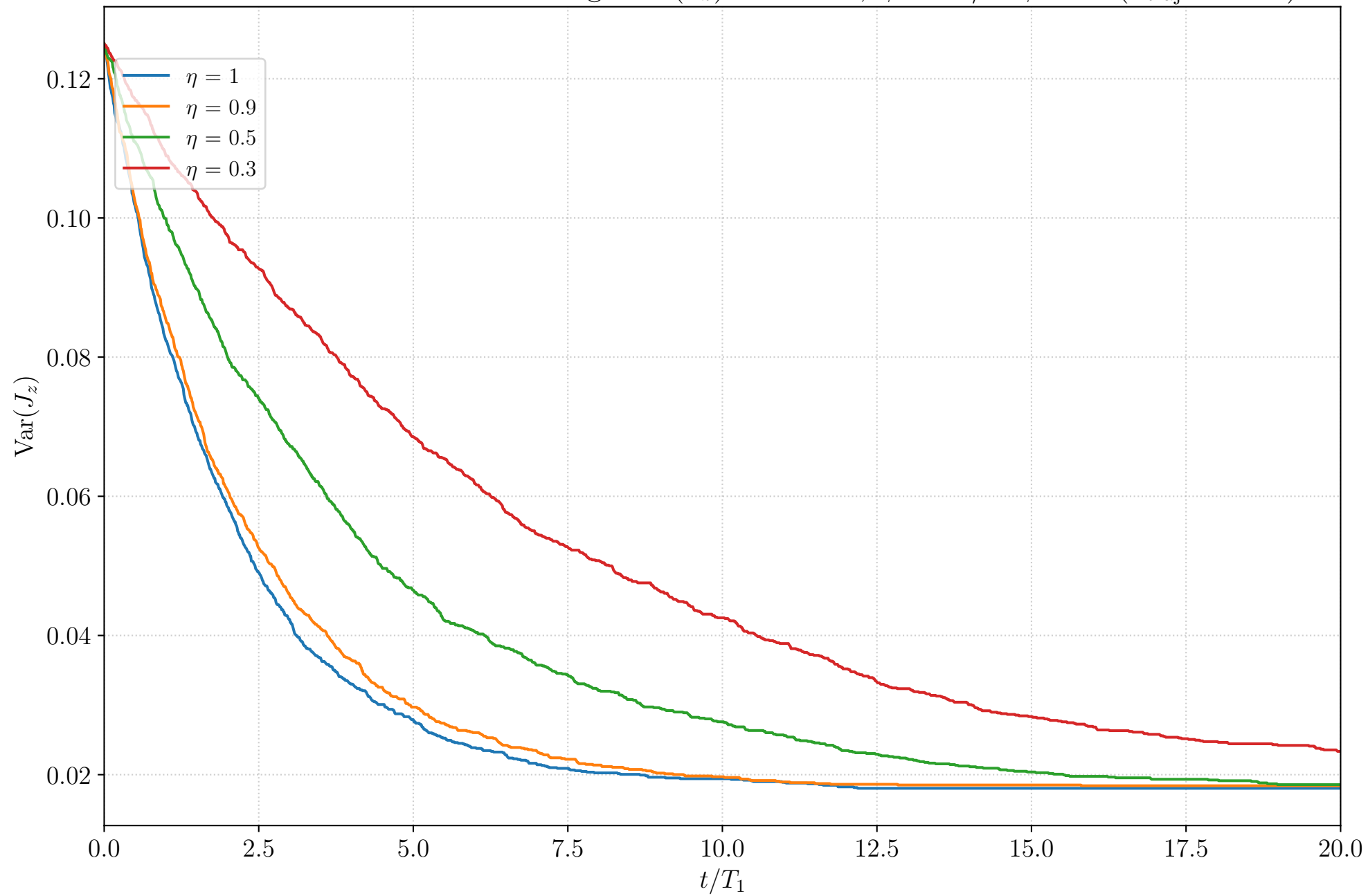
Inefficient Photodetection: Average \text{Var}(J_z) over time, \phi_1 = \pi/2 \phi_2 = 0 ( n_{\text{traj}} = 1000 )
