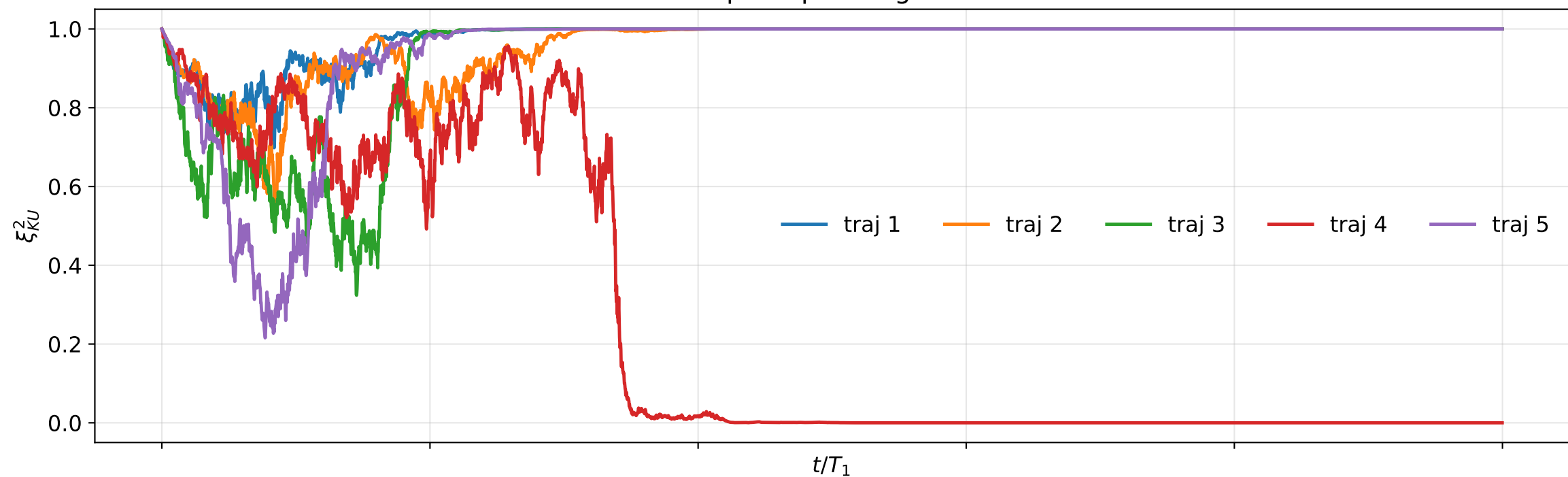
Spin Squeezing Wineland
