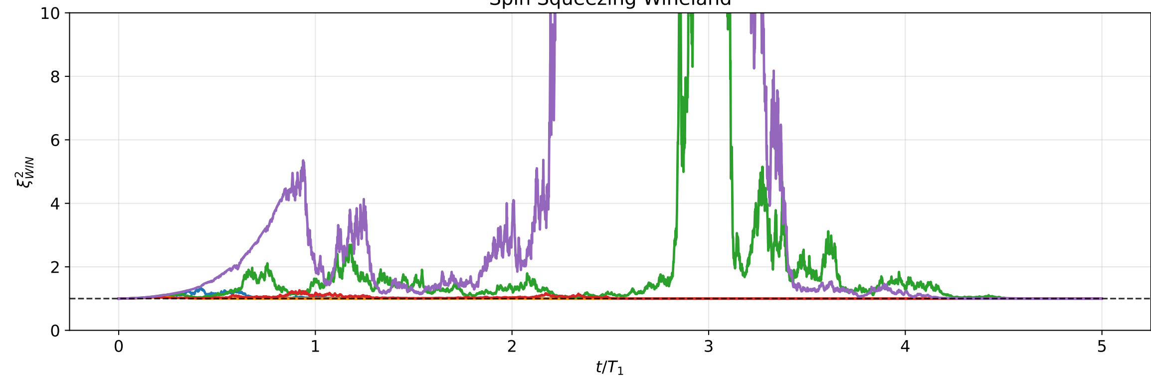
Spin Squeezing Wineland
