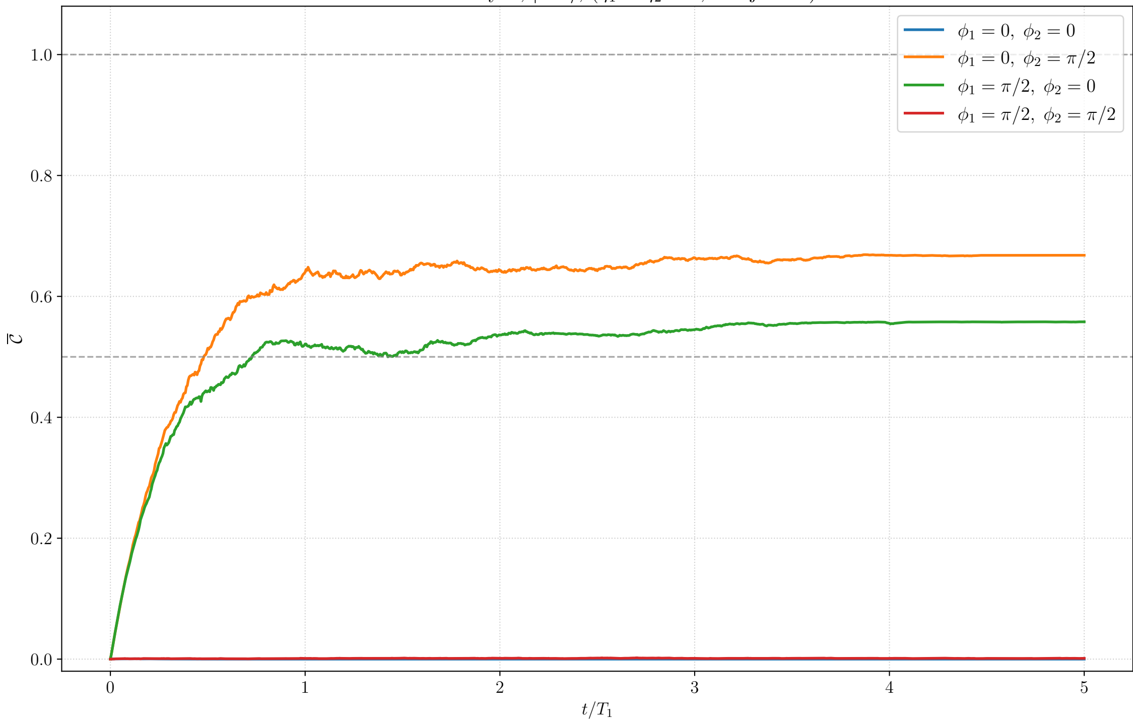
Ideal homodyne, |++\rangle , ( \eta_1 = \eta_2 = 1 , ntraj= 100)
