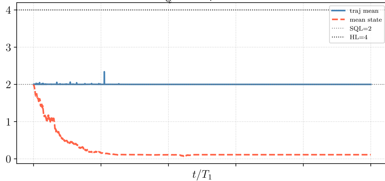
F_Q^{\max} — \eta = 0.6
