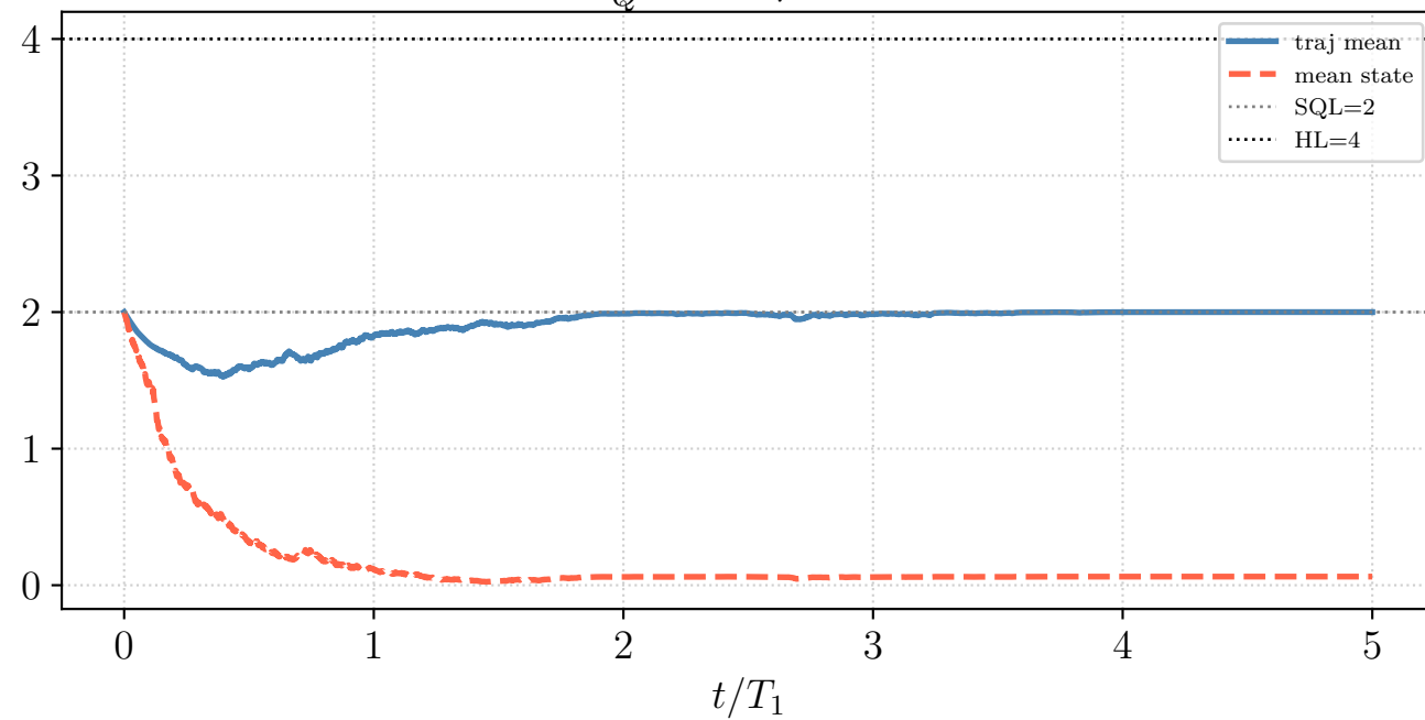
F_Q^{\max} — \eta = 0.6
