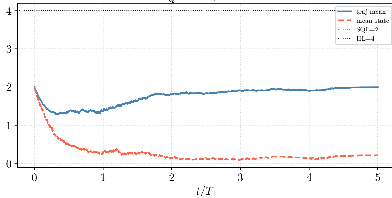
F_Q^{\max} — \eta = 0.4
