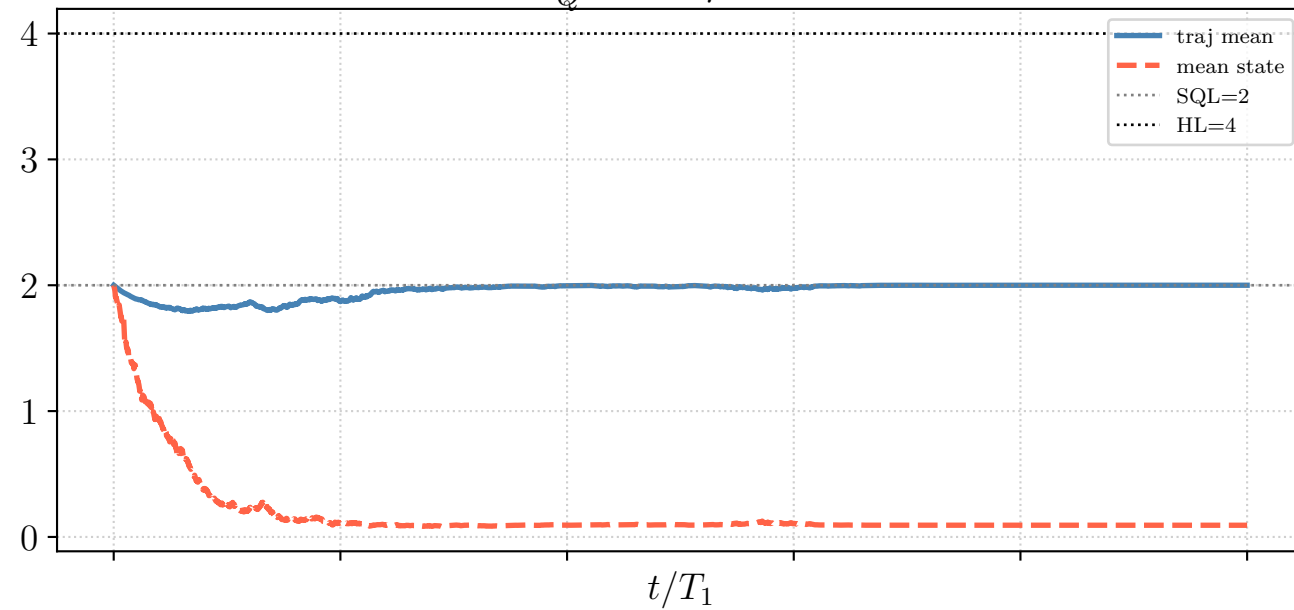
F_Q^{\max} — \eta = 0.4
