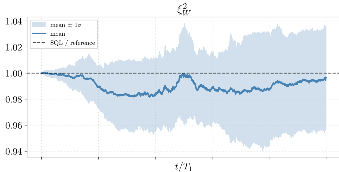
Ideal trajectories — ensemble mean \pm 1\sigma (ntraj=30)
