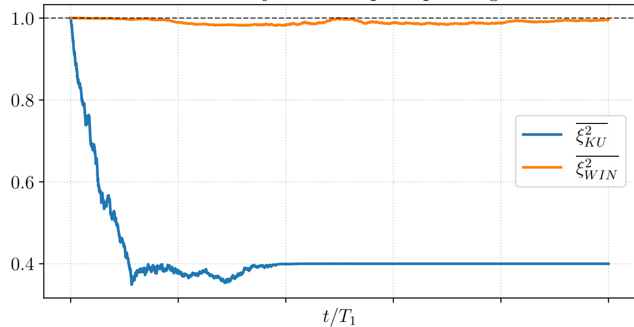
Ideal trajectories: Variance on J_z
