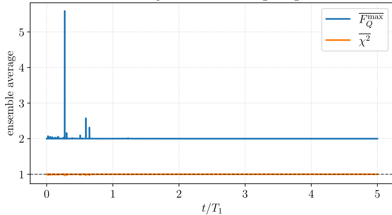
Ideal trajectories: Metrological gain
