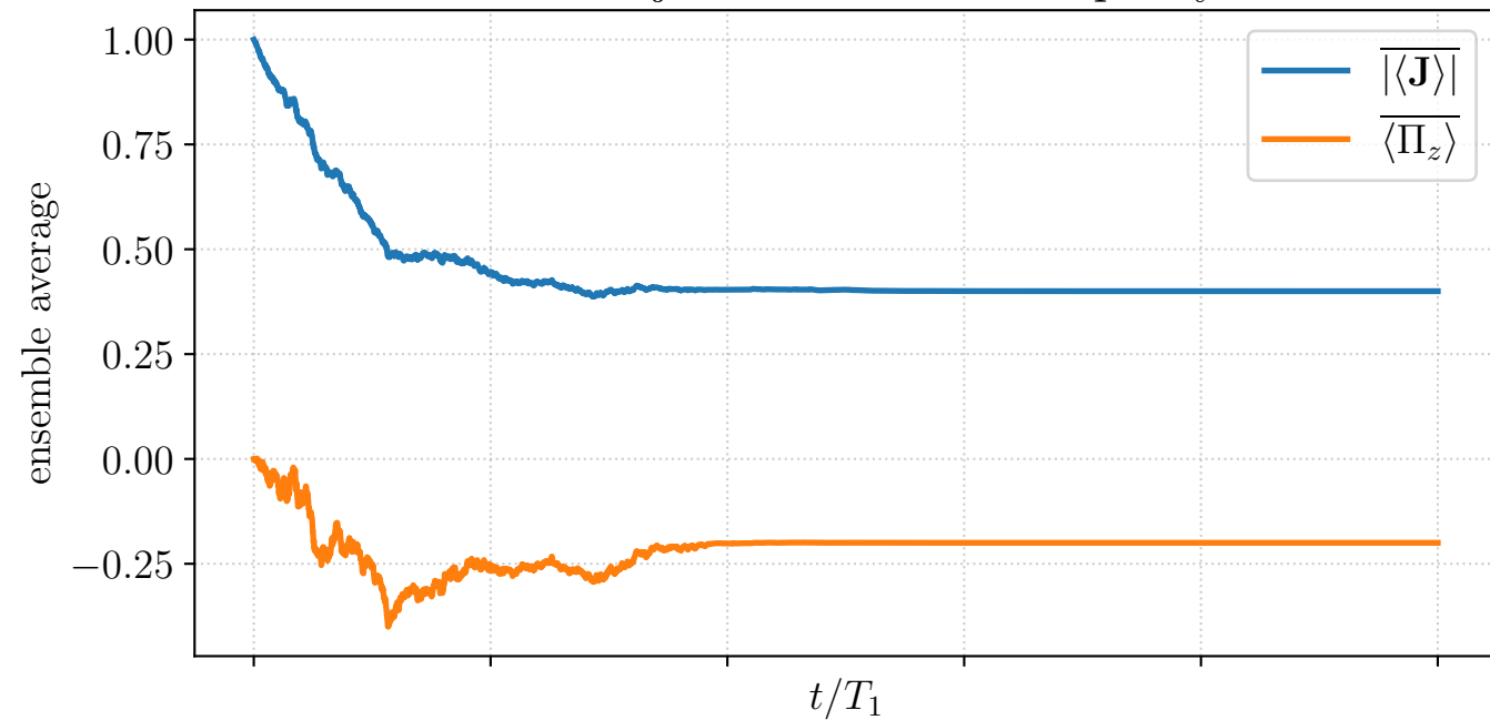
Ideal trajectories: Metrological gain
