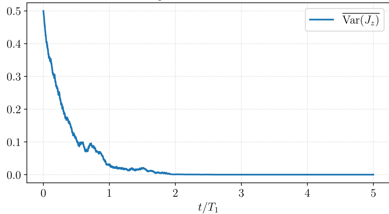
Ideal trajectories: Variance on J_z
