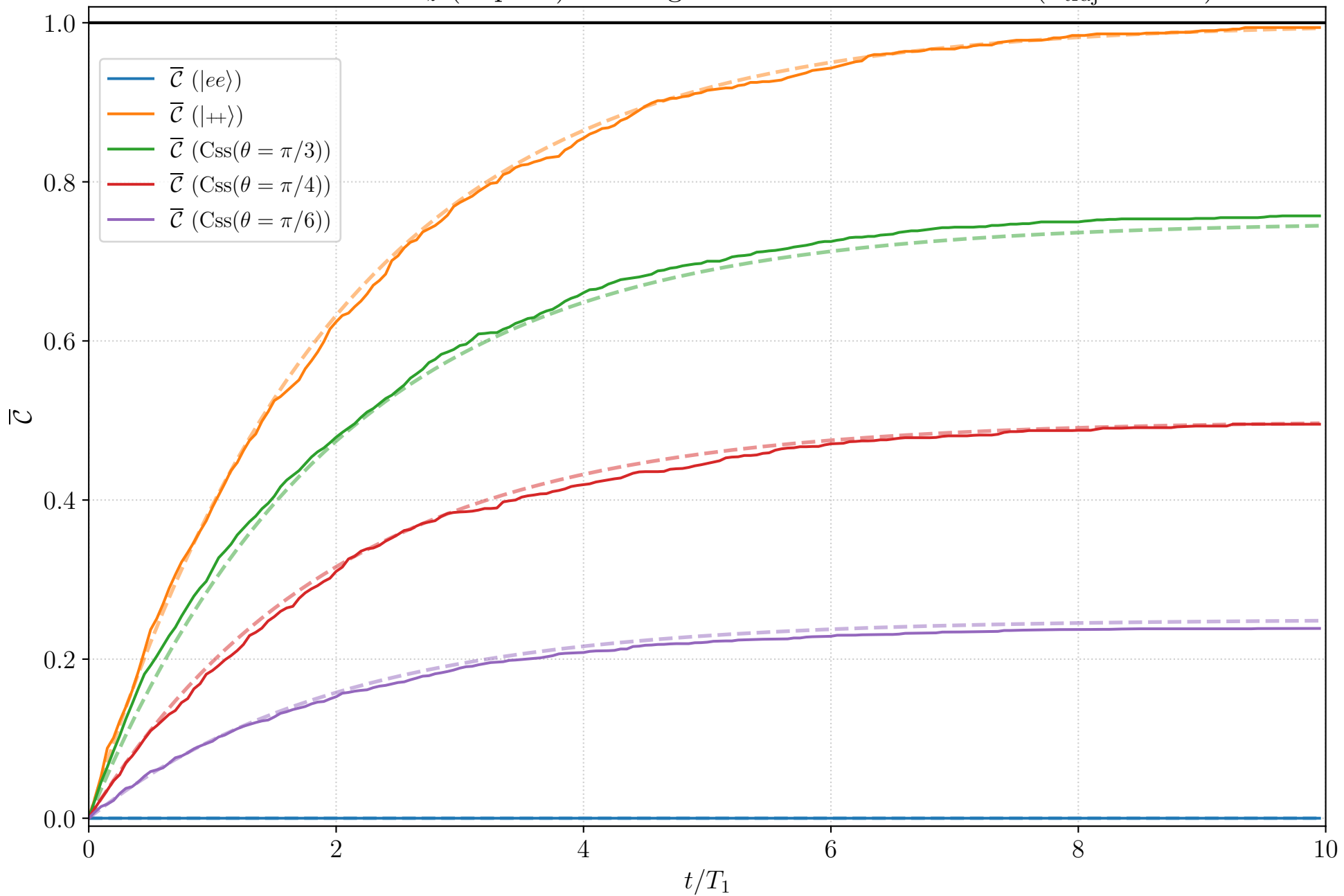
Photodetection J_z (2 qubit): Average concurrence \bar{\mathcal{C}} over time ( n_{\text{traj}} = 1000 )
