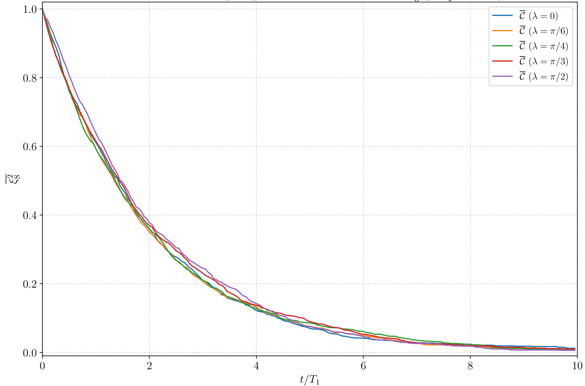
Photodetection J_z |++\rangle : Average Spin Squeezing \overline{\xi_S^2} ( n_{\text{traj}} = 1000 )
