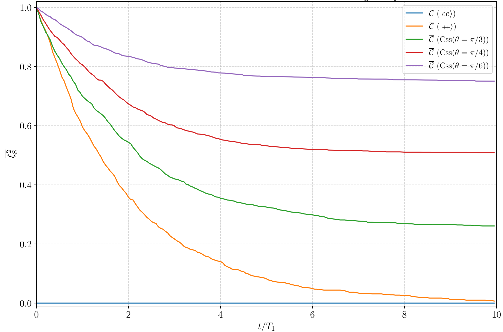
Photodetection J_z (2 qubit): Average Spin Squeezing \overline{\xi_S^2} ( n_{\text{traj}} = 1000 )
