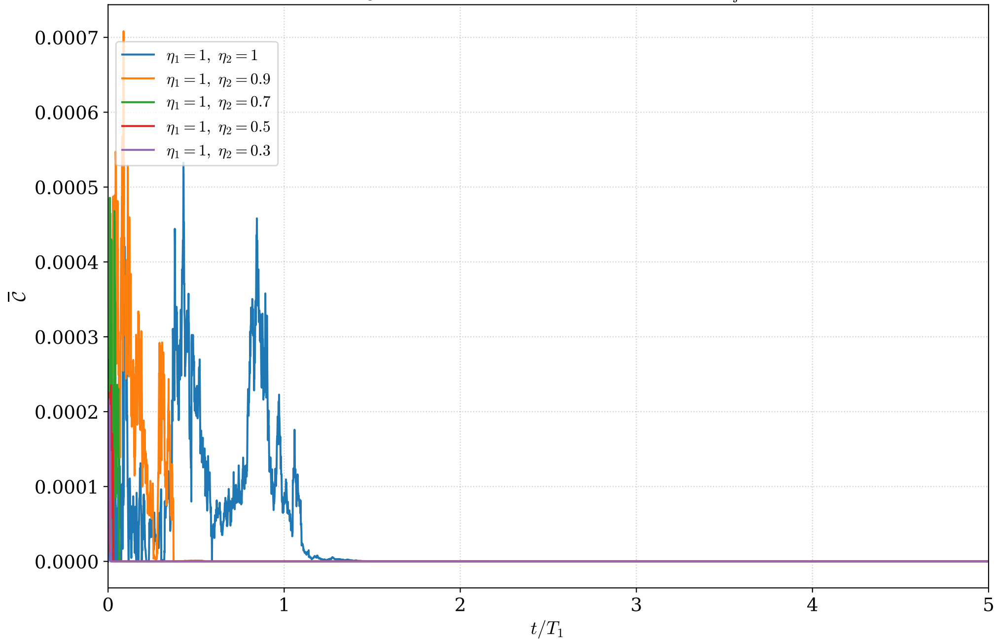
Homodyne J_z (N=2): \bar{\mathcal{C}} , \phi_1 = 0 \phi_2 = 0 ( n_{\text{traj}} = 20 )
