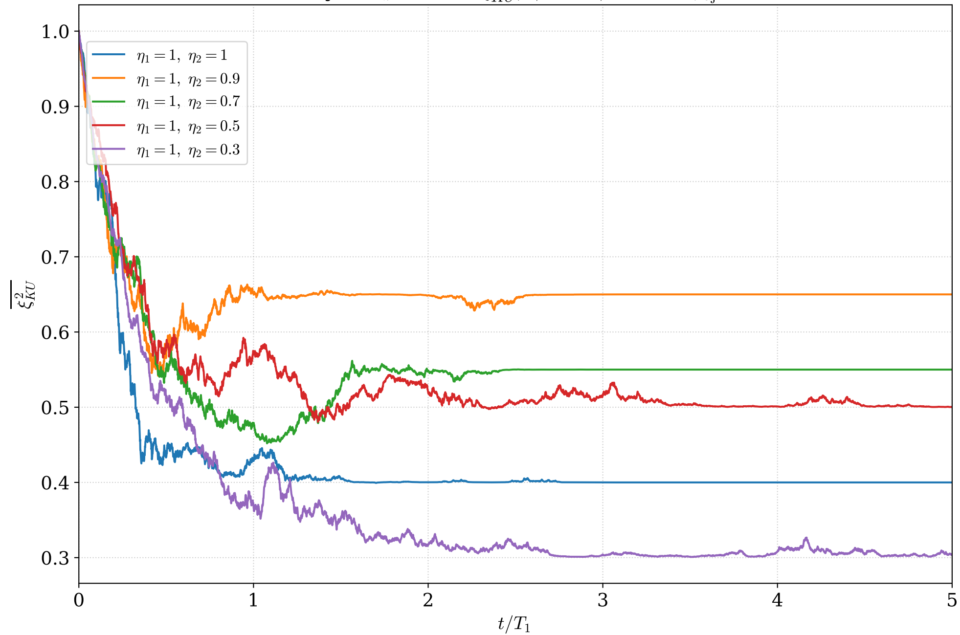
Homodyne J_z (N=2): \overline{\xi_{KU}^2} , \phi_1 = 0 \phi_2 = 0 ( n_{\text{traj}} = 20 )
