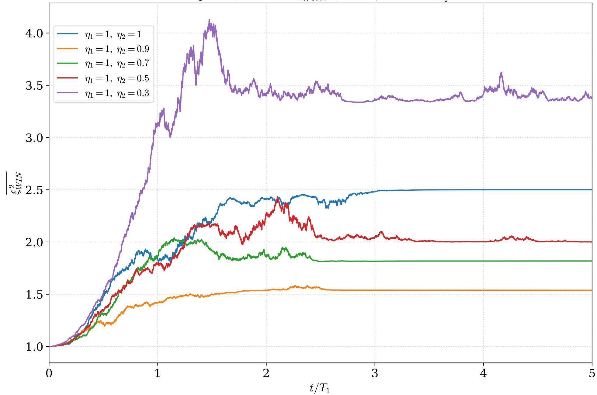
Homodyne J_z (N=2): \overline{\xi_{WIN}^2} , \phi_1 = 0 \phi_2 = 0 ( n_{\text{traj}} = 20 )
