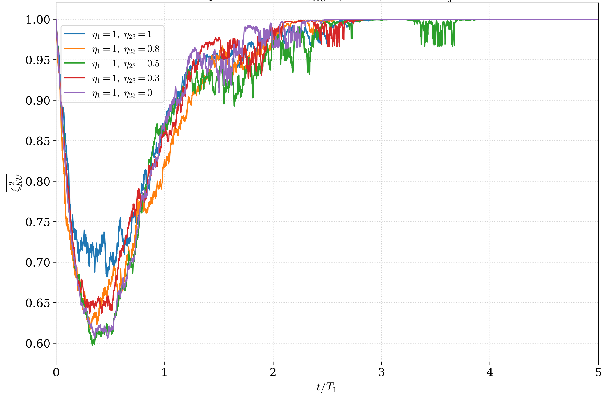
Homodyne J_z (N=3): \overline{\xi_{KU}^2} , \phi_1 = 0 \phi_2 = 0 ( n_{\text{traj}} = 20 )
