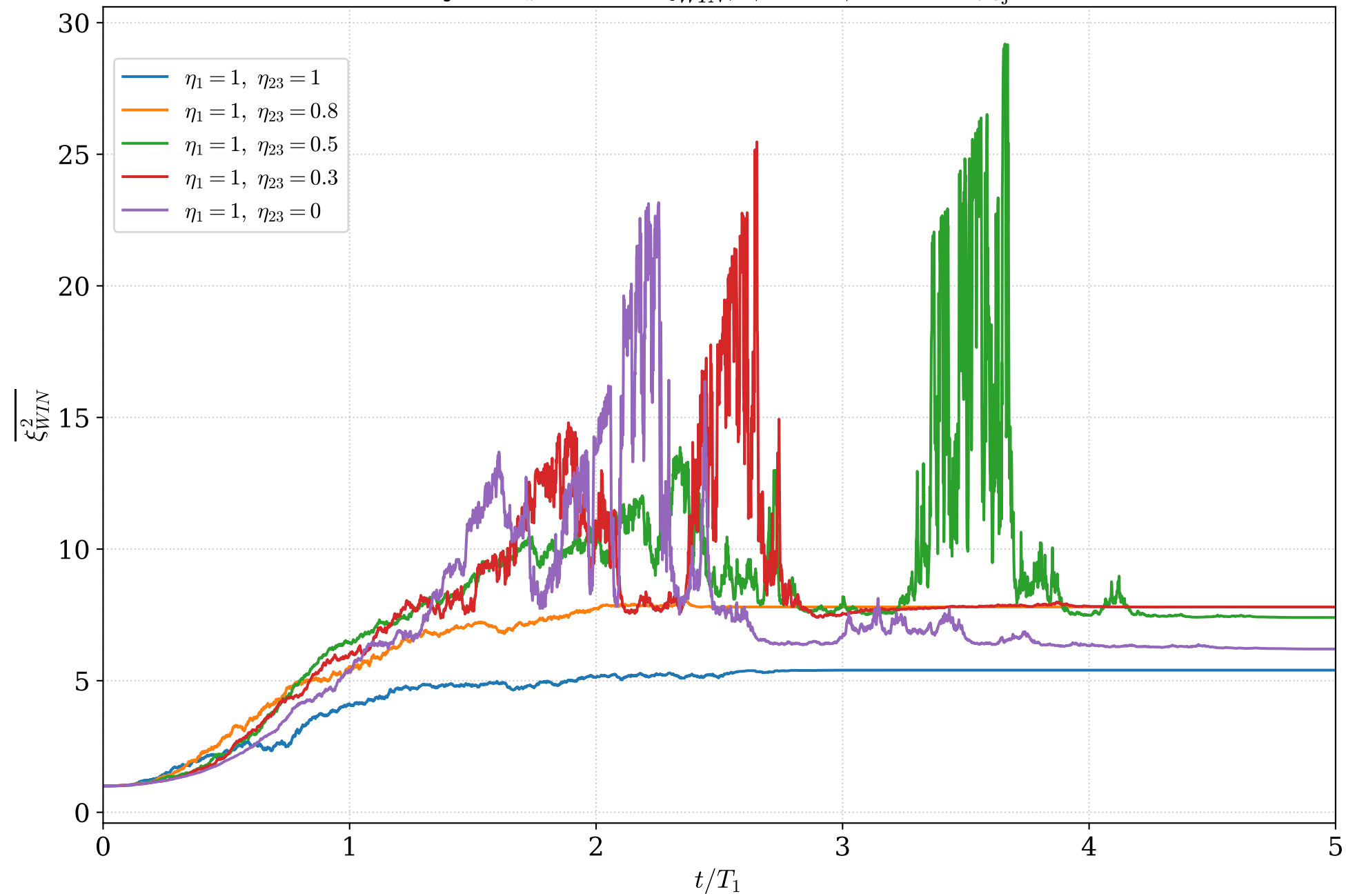
Homodyne J_z (N=3): \overline{\xi_{WIN}^2} , \phi_1 = 0 \phi_2 = 0 ( n_{\text{traj}} = 20 )
