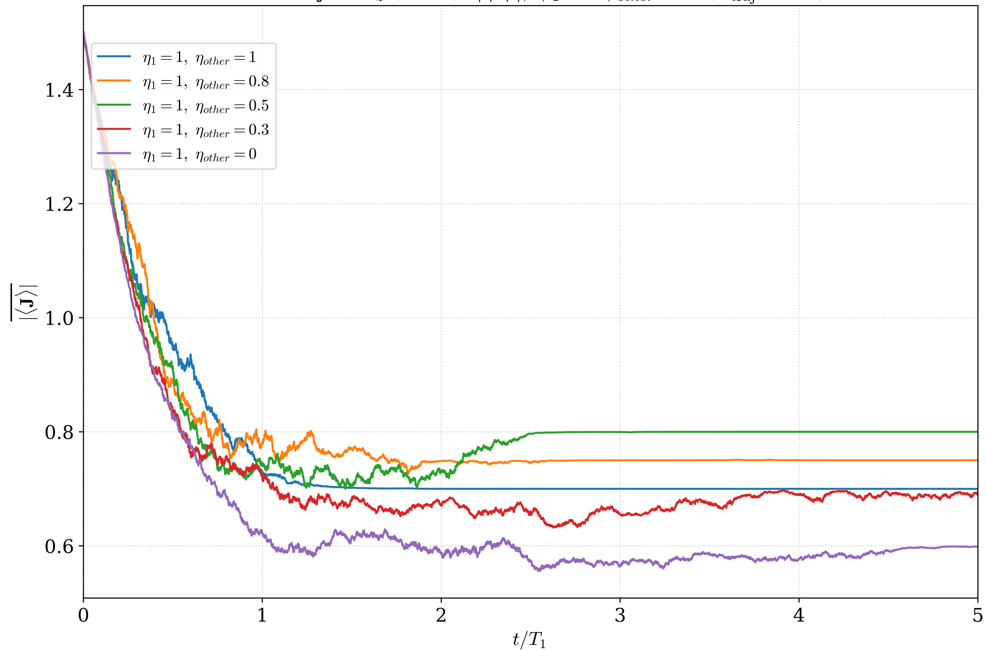
Homodyne J_z (N=3): |\overline{\langle \mathbf{J} \rangle}| , \phi_1 = 0 \phi_{other} = 0 ( n_{\text{traj}} = 20 )
