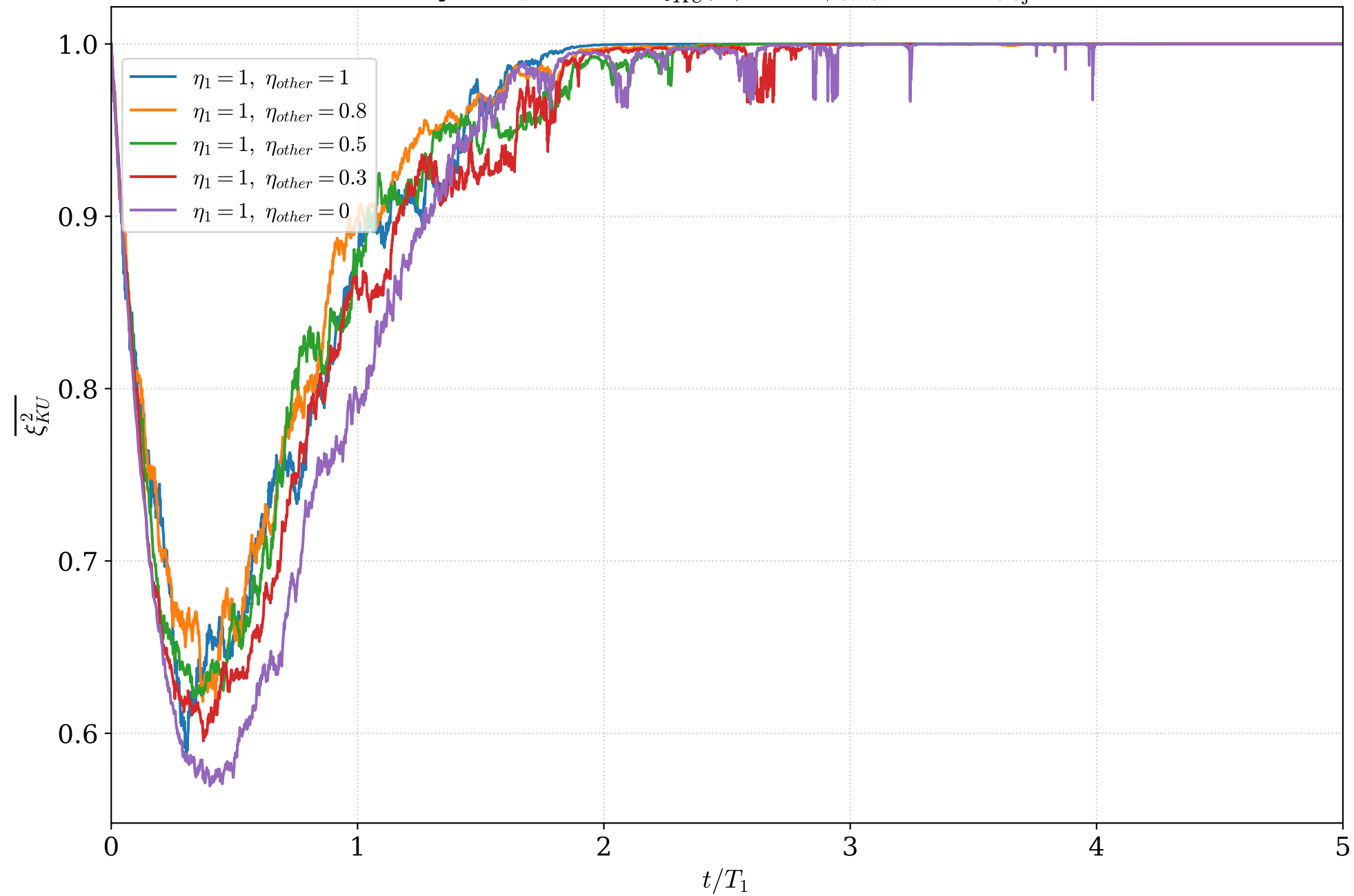
Homodyne J_z (N=3): \overline{\xi_{KU}^2} , \phi_1 = 0 \phi_{other} = 0 ( n_{\text{traj}} = 20 )
