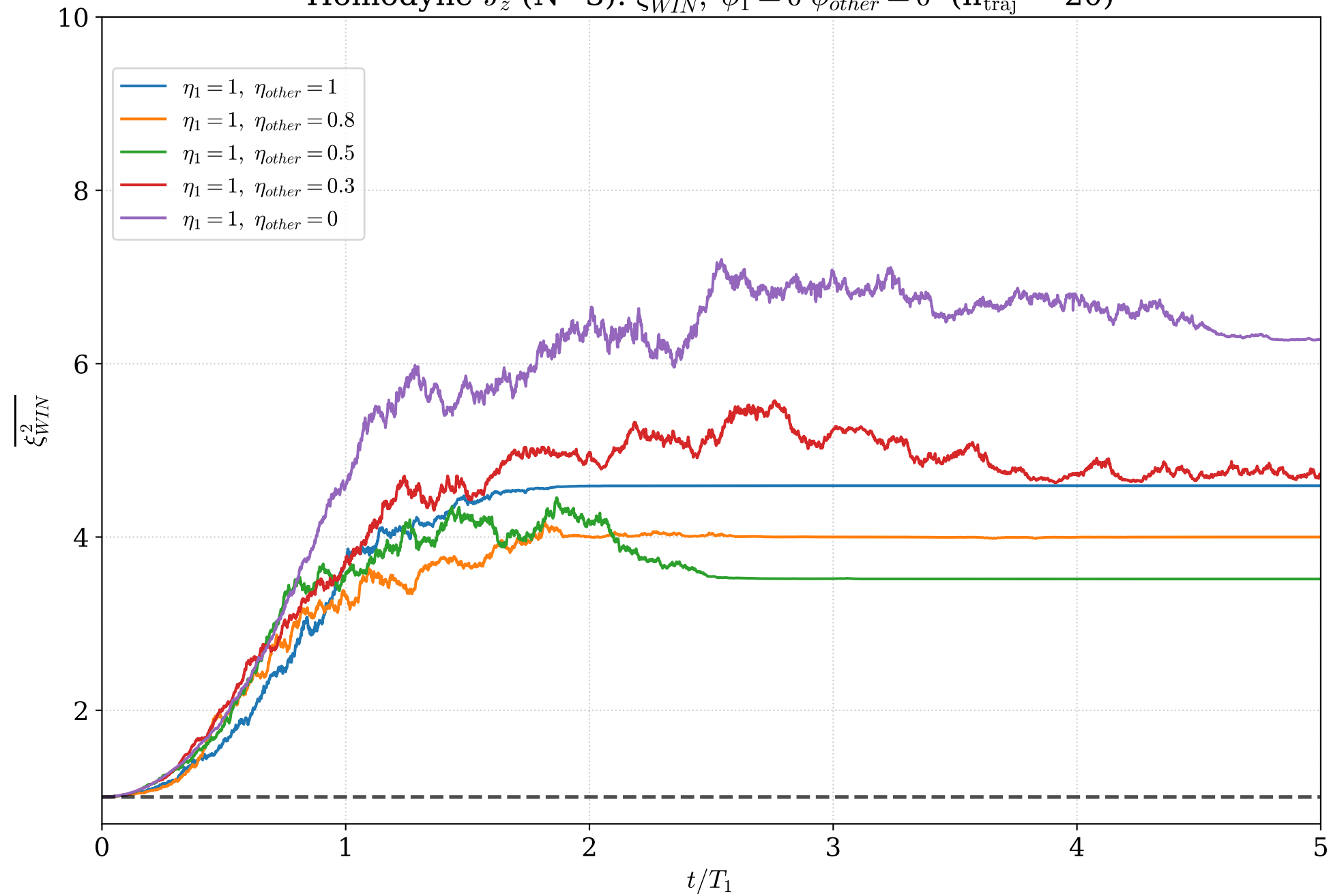
Homodyne J_z (N=3): \overline{\xi_{WIN}^2} , \phi_1 = 0 \phi_{other} = 0 ( n_{traj} = 20 )
