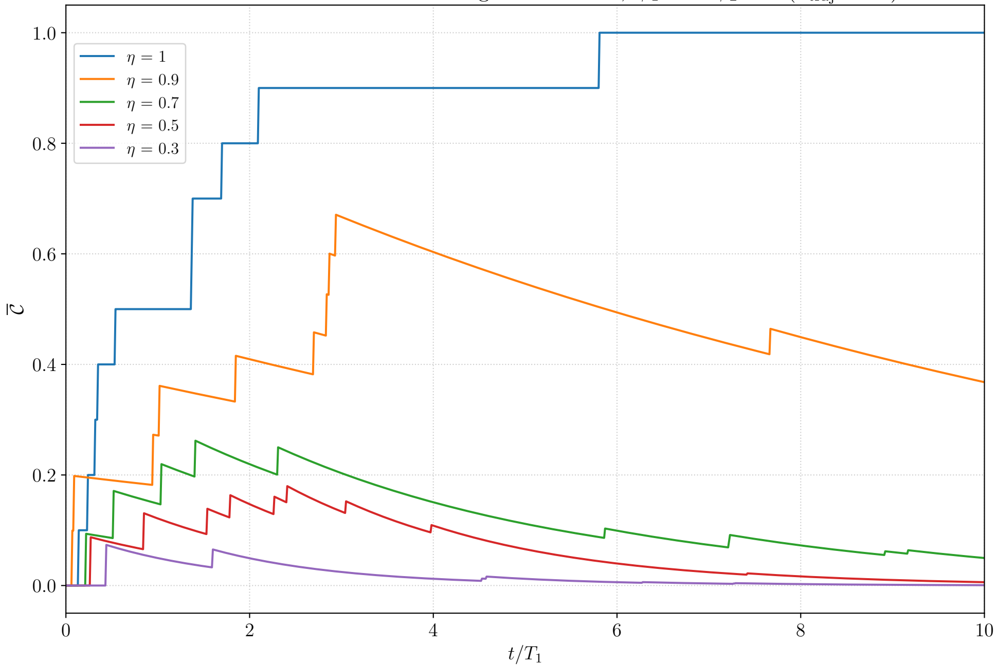
Inefficient Photodetection: Average \bar{\mathcal{C}} over time, \phi_1 = 0 \phi_2 = 0 ( n_{\text{traj}} = 10 )
