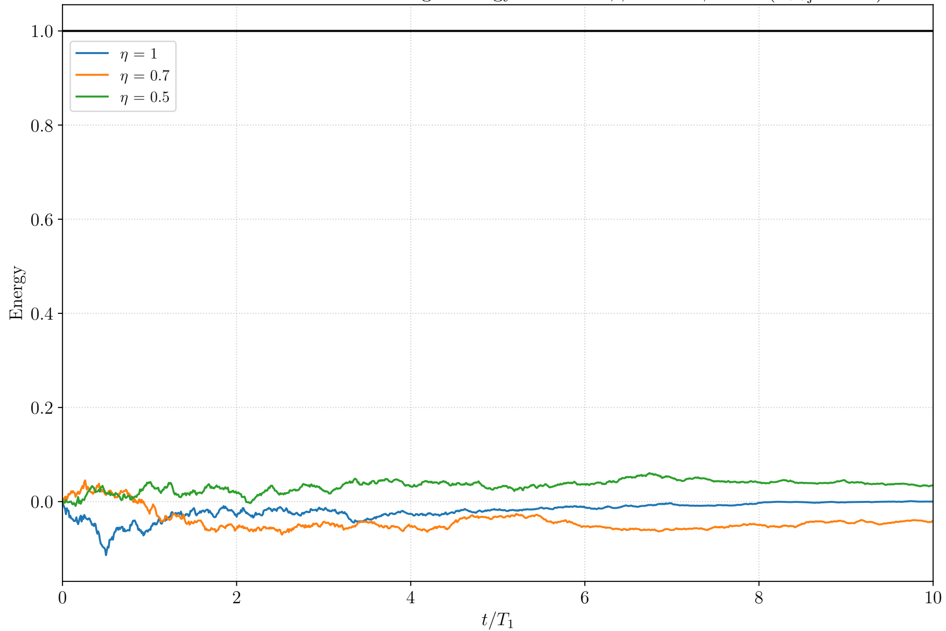
Inefficient Photodetection: Average Energy over time, \phi_1 = 0 \phi_2 = 0 ( n_{\text{traj}} = 100 )
