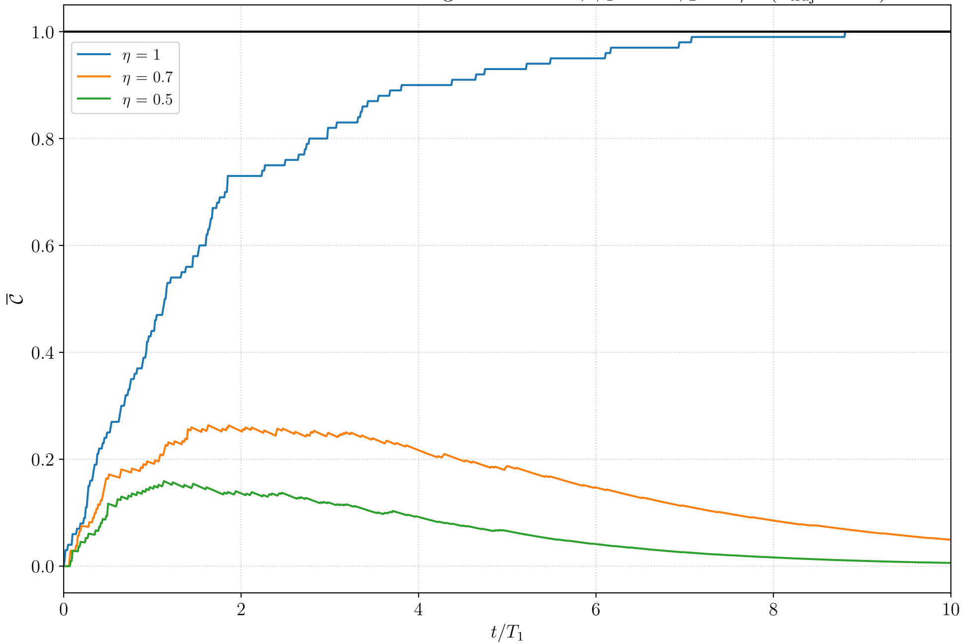
Inefficient Photodetection: Average \bar{\mathcal{C}} over time, \phi_1 = 0 \phi_2 = \pi/2 ( n_{\text{traj}} = 100 )
