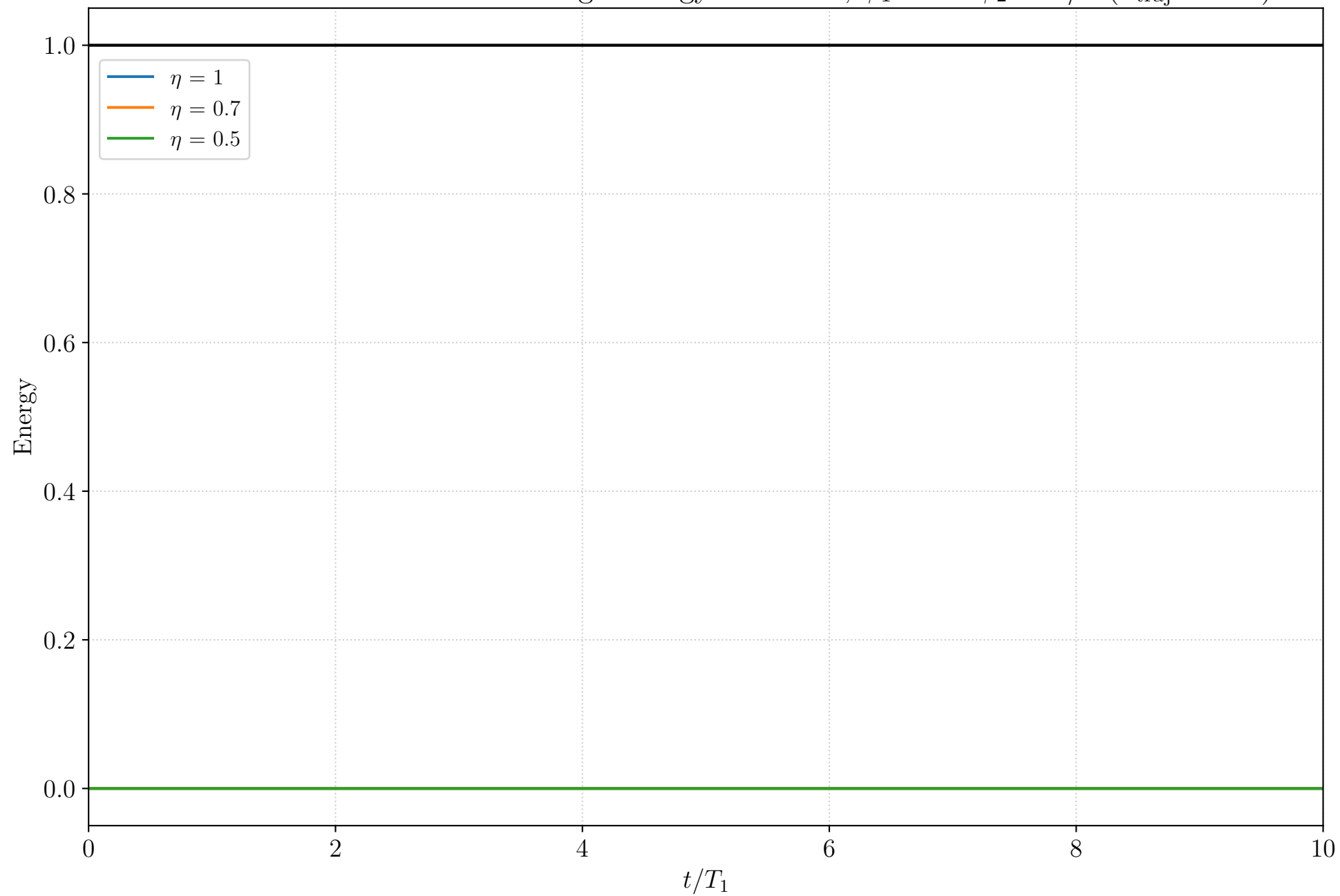
Inefficient Photodetection: Average Energy over time, \phi_1 = 0 \phi_2 = \pi/2 ( n_{\text{traj}} = 100 )
