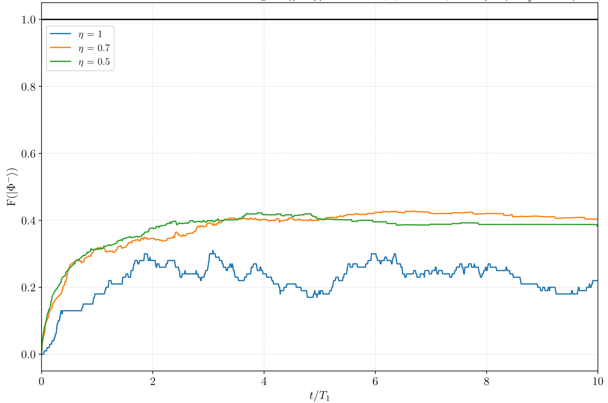
Inefficient Photodetection: Average F(|\Phi^-\rangle) over time, \phi_1 = 0 \phi_2 = \pi/2 ( n_{\text{traj}} = 100 )
