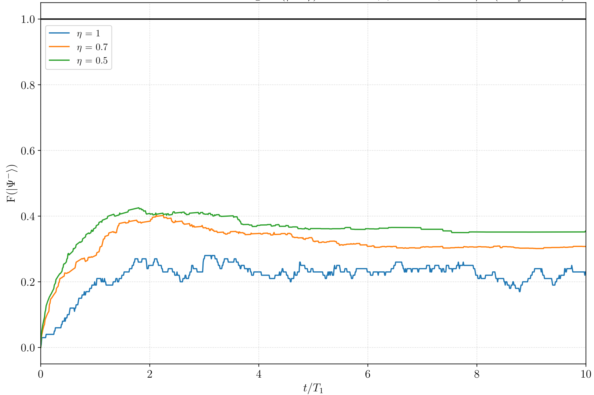
Inefficient Photodetection: Average F(|\Psi^-\rangle) over time, \phi_1 = 0 \phi_2 = \pi/2 ( n_{\text{traj}} = 100 )
