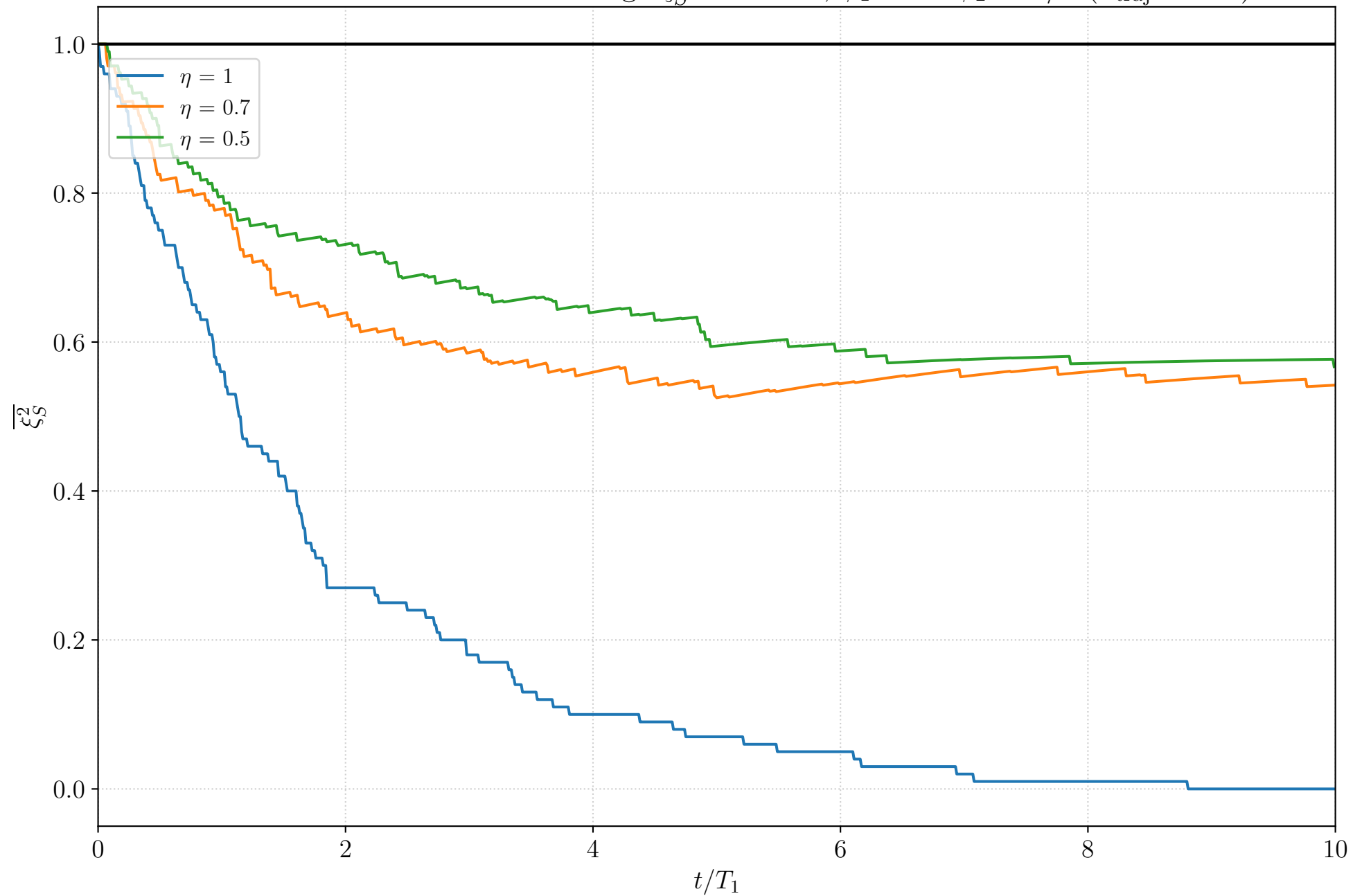
Inefficient Photodetection: Average \overline{\xi_S^2} over time, \phi_1 = 0 \phi_2 = \pi/2 ( n_{\text{traj}} = 100 )
