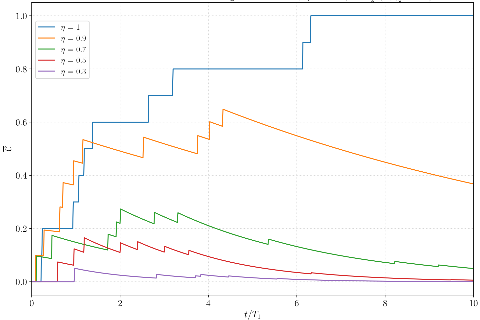
Inefficient Photodetection: Average \bar{\mathcal{C}} over time, \phi_1 = 0 \phi_2 = \frac{\pi}{2} ( n_{\text{traj}} = 10 )
