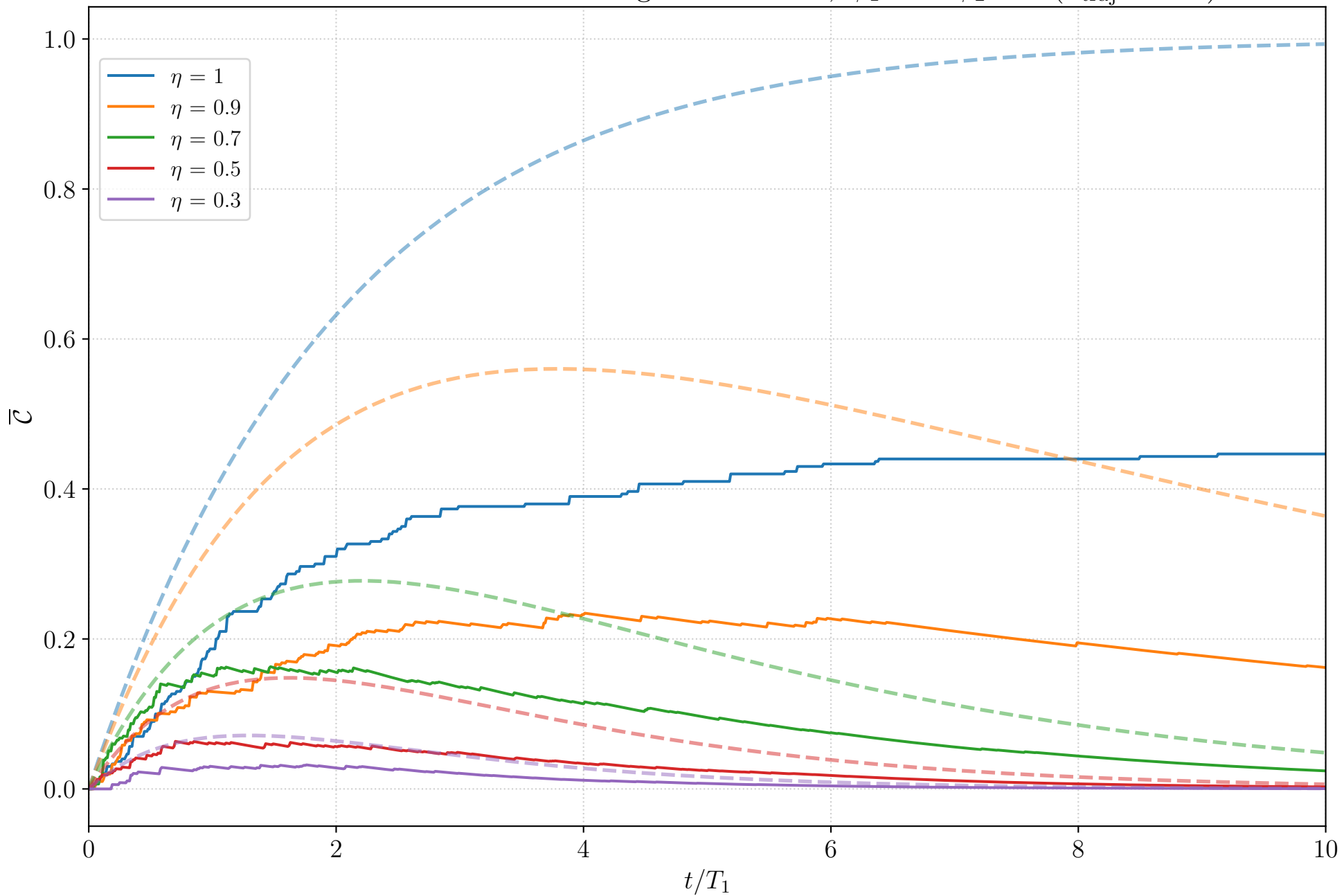
Inefficient Photodetection: Average \bar{\mathcal{C}} over time, \phi_1 = 0 \phi_2 = 0 ( n_{\text{traj}} = 100 )
