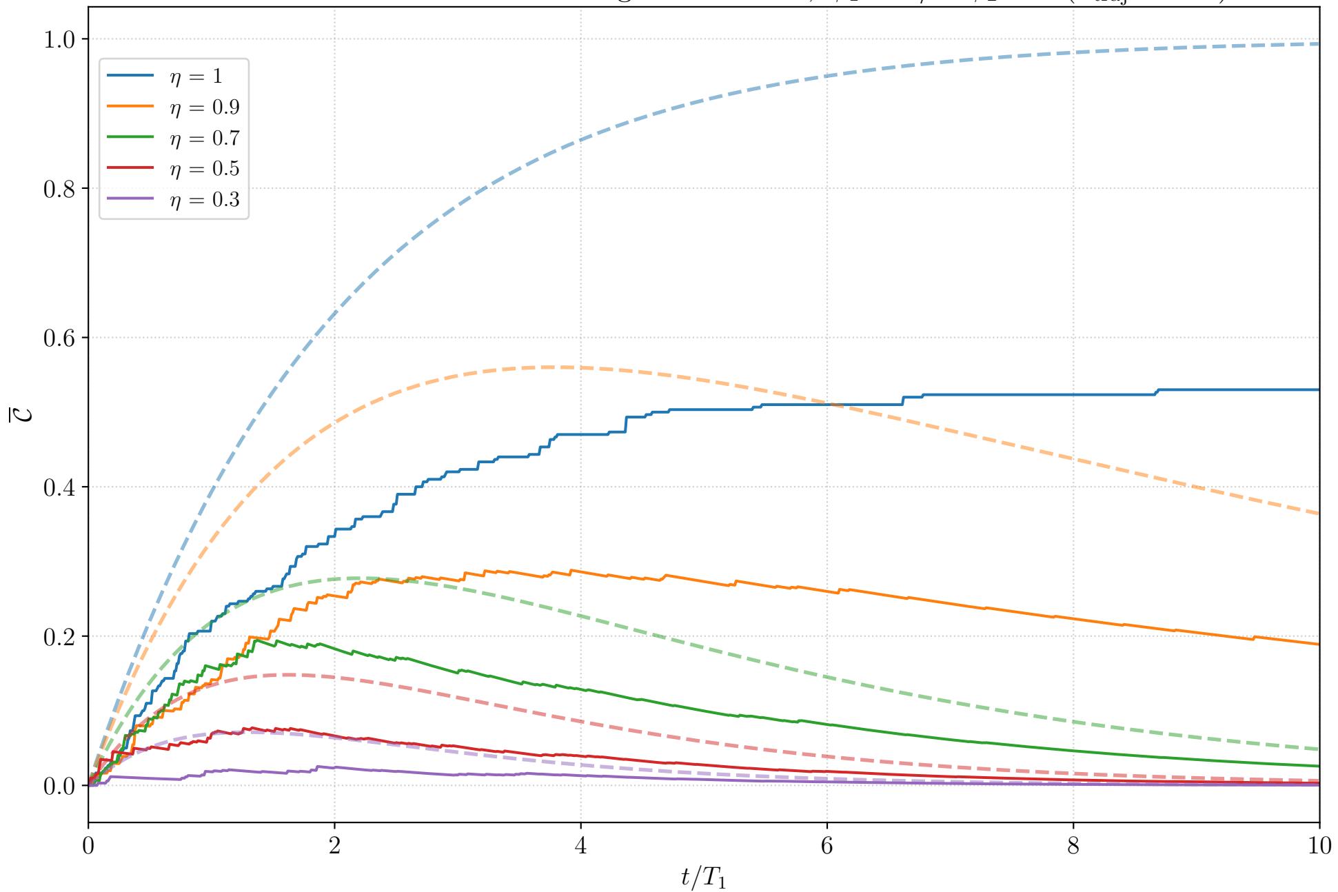
Inefficient Photodetection: Average \bar{\mathcal{C}} over time, \phi_1 = \pi/2 \phi_2 = 0 ( n_{\text{traj}} = 100 )
